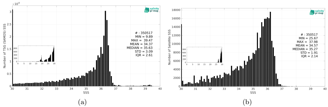
Figure 3: Histograms of SSS from TSG (SAMOS) (a) and SMOS SSS L3 v335 - Monthly - 25 km (CATDS-CPDC) (b) considering all match-up pairs per bins of 0.1 over the Mississippi river plume Pi-MEP region and for the full satellite product period.
