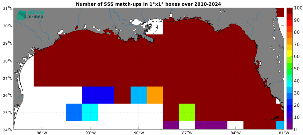
Figure 5: Number of SSS match-ups between TSG (SAMOS) SSS and the SMOS SSS L3 v335 - Monthly - 25 km (CATDS-CPDC) SSS product for the Mississippi river plume Pi-MEP region over 1^\circ \times 1^\circ boxes and for the full satellite product period.
