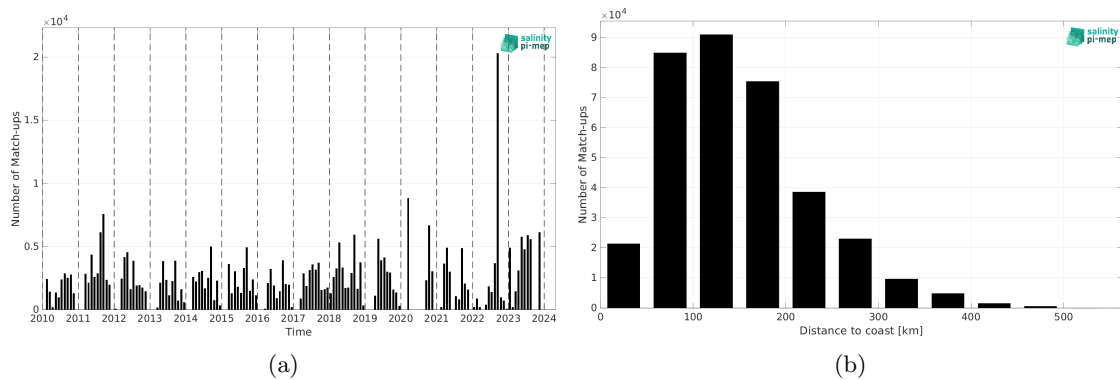
Figure 2: Number of match-ups between TSG (SAMOS) and SMOS SSS L3 v335 - Monthly - 25 km (CATDS-CPDC) SSS as a function of time (a) and as function of the distance to coast (b) over the Mississippi river plume Pi-MEP region and for the full satellite product period.
