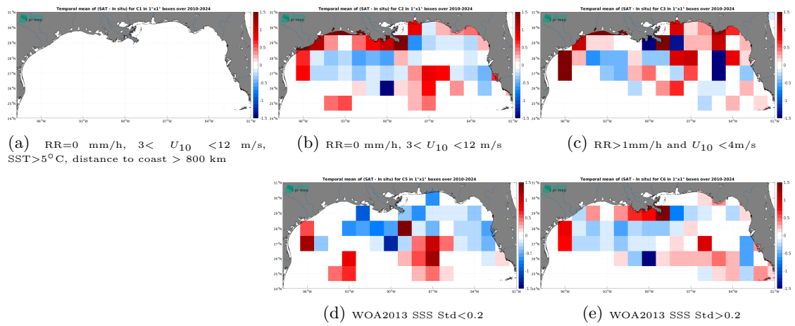
Figure 14: Temporal mean gridded over spatial boxes of size 1^\circ \times 1^\circ of \Delta SSS (SMOS SSS L3 v335 - Monthly - 25 km (CATDS-CPDC) - TSG (SAMOS)) for 5 different subdatasets corresponding to: RR=0 mm/h, 3 < U_{10} < 12 m/s, SST > 5°C, distance to coast > 800 km (a), RR=0 mm/h, 3 < U_{10} < 12 m/s (b), RR > 1 mm/h and U_{10} < 4 m/s (c), WOA2013 SSS Std < 0.2 (d), WOA2013 SSS Std > 0.2 (e).
