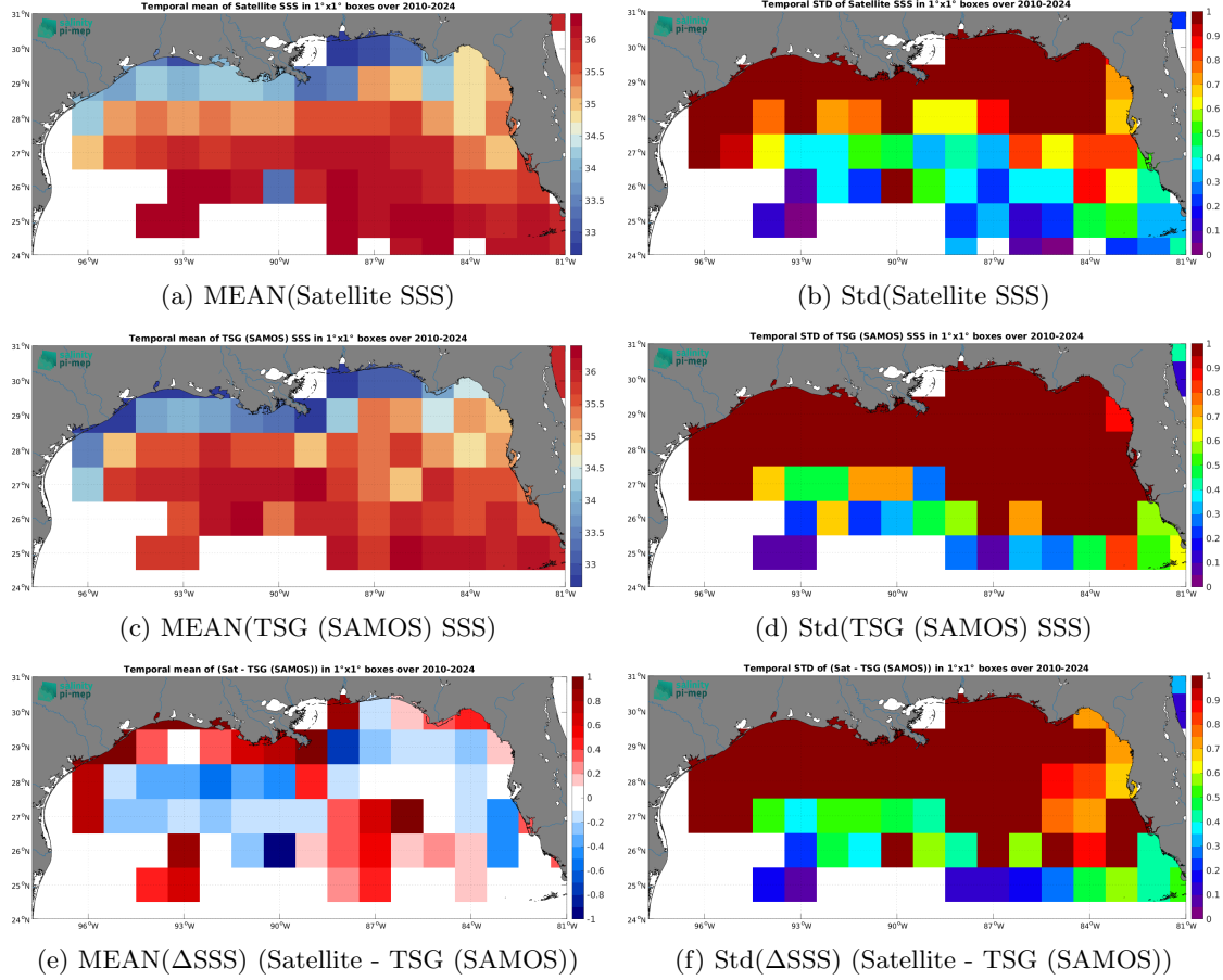
Figure 7: Temporal mean (left) and Std (right) of SSS from SMOS SSS L3 v335 - Monthly - 25 km (CATDS-CPDC) (top), TSG (SAMOS) (middle), and of \Delta\text{SSS} (Satellite - TSG (SAMOS)). Only match-up pairs are used to generate these maps.
