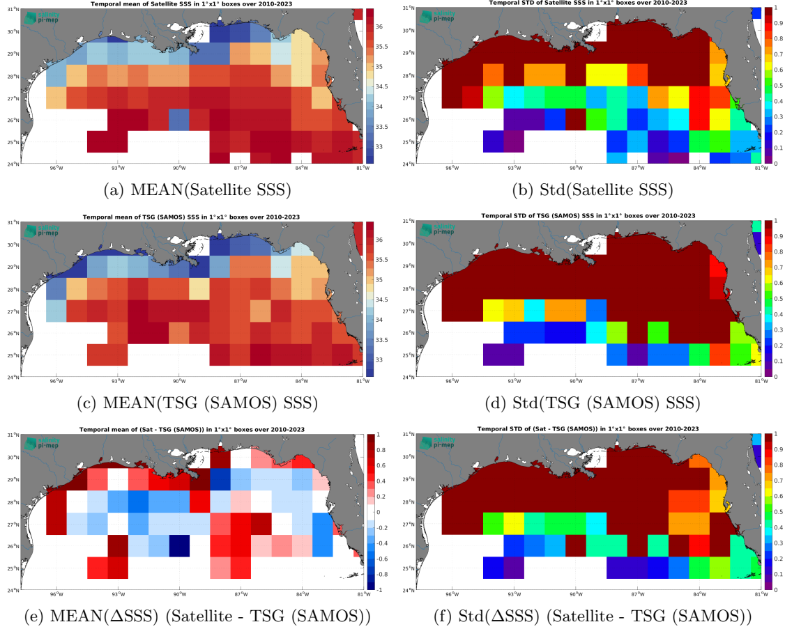
Figure 6: Temporal mean (left) and Std (right) of SSS from SMOS SSS L3 v335 - Monthly - 25 km (CATDS-CPDC) (top), TSG (SAMOS) (middle), and of \Delta\text{SSS} (Satellite - TSG (SAMOS)). Only match-up pairs are used to generate these maps.
