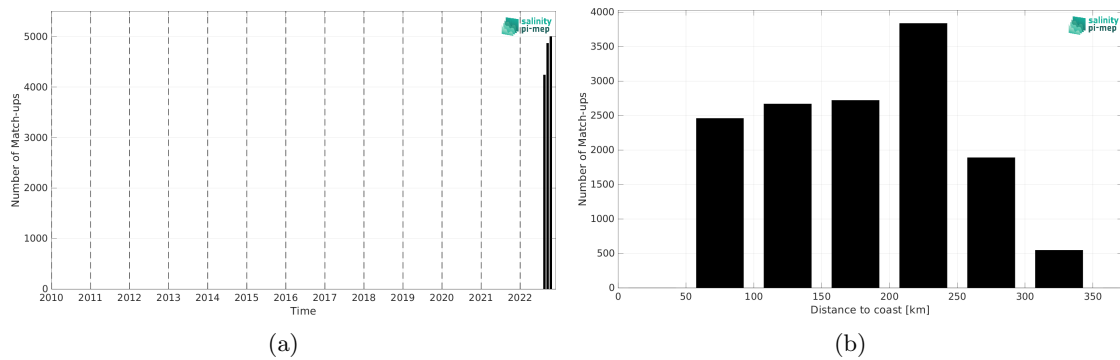
Figure 2: Number of match-ups between Saildrone and SMOS SSS L3 v335 - Monthly - 25 km (CATDS-CPDC) SSS as a function of time (a) and as function of the distance to coast (b) over the Mississippi river plume Pi-MEP region and for the full satellite product period.
