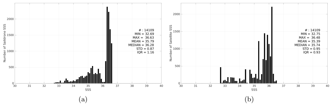
Figure 3: Histograms of SSS from Saildrone (a) and SMOS SSS L3 v335 - Monthly - 25 km (CATDS-CPDC) (b) considering all match-up pairs per bins of 0.1 over the Mississippi river plume Pi-MEP region and for the full satellite product period.
