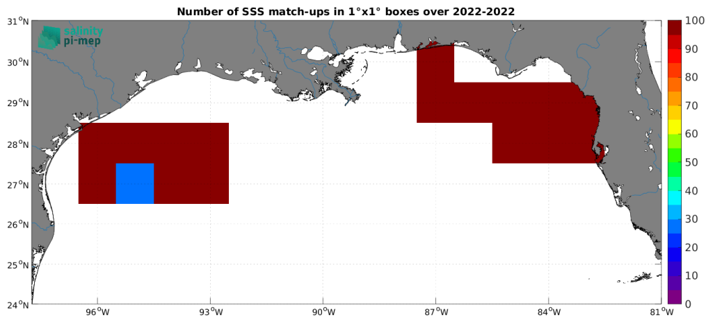
Figure 5: Number of SSS match-ups between Saildrone SSS and the SMOS SSS L3 v335 - Monthly - 25 km (CATDS-CPDC) SSS product for the Mississippi river plume Pi-MEP region over 1^\circ \times 1^\circ boxes and for the full satellite product period.
