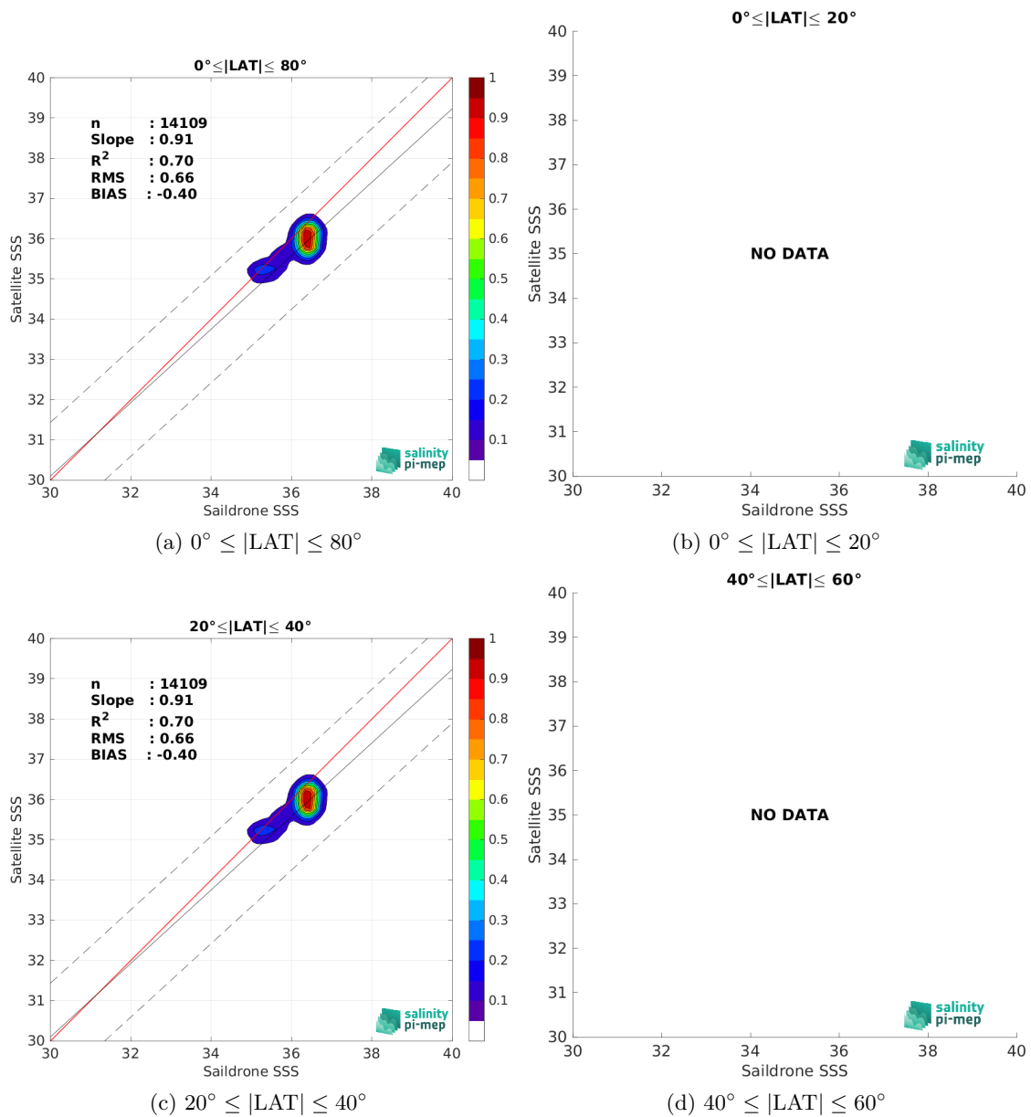
Figure 9: Contour maps of the concentration of SMOS SSS L3 v335 - Monthly - 25 km (CATDS-CPDC) SSS (y-axis) versus Saïdrone SSS (x-axis) at match-up pairs for different latitude bands. For each plot, the red line shows x=y . The black thin and dashed lines indicate a linear fit through the data cloud and the \pm 95\% confidence levels, respectively. The number match-up pairs n , the slope and R^2 coefficient of the linear fit, the root mean square (RMS) and the mean bias between satellite and in situ data are indicated for each latitude band in each plots.
