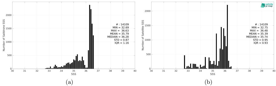
Figure 2: Histograms of SSS from Sairdrone (a) and SMOS SSS L3 v335 - Monthly - 25 km (CATDS-CPDC) (b) considering all match-up pairs per bins of 0.1 over the Mississippi river plume Pi-MEP region and for the full satellite product period.
