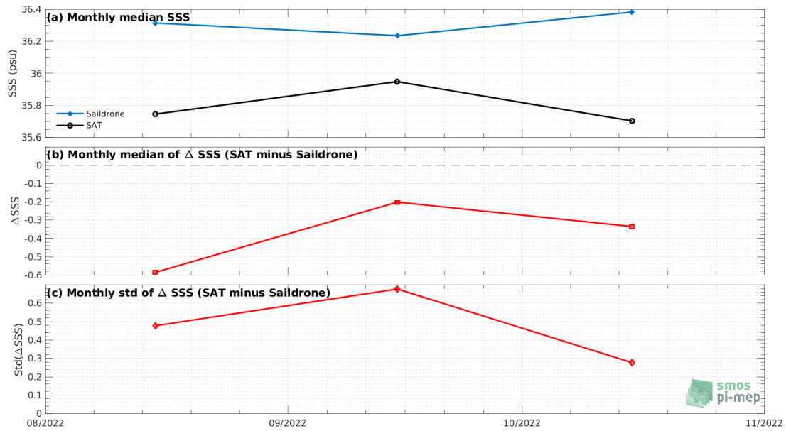
Figure 7: Time series of the monthly median SSS (top), median of \Delta SSS (Satellite - SSS in situ) and Std of \Delta SSS (Satellite - SSS in situ) over the Mississippi river plume Pi-MEP region considering all match-ups collected by the Pi-MEP.
