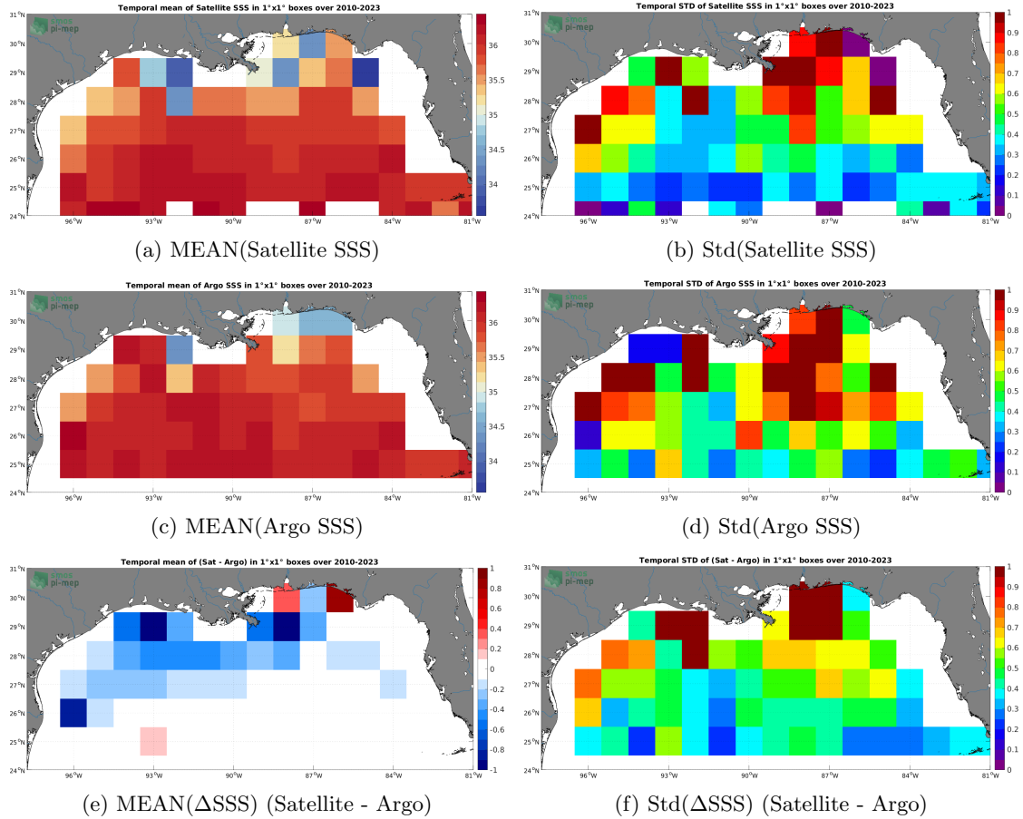
Figure 6: Temporal mean (left) and Std (right) of SSS from SMOS SSS L3 v335 - Monthly - 25 km (CATDS-CPDC) (top), Argo (middle), and of \Delta\text{SSS} (Satellite - Argo). Only match-up pairs are used to generate these maps.
