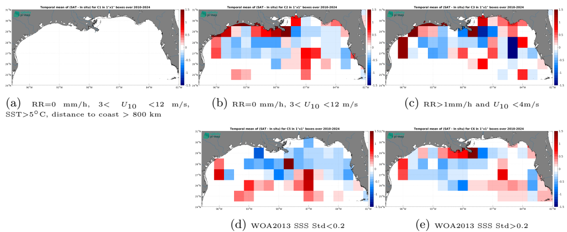
Figure 14: Temporal mean gridded over spatial boxes of size 1^\circ \times 1^\circ of \Delta SSS (SMOS SSS L3 v335 - 10 Days - 25 km (CATDS-CPDC) - TSG (SAMOS)) for 5 different subdatasets corresponding to: RR=0 mm/h, 3 < U_{10} < 12 m/s, SST > 5°C, distance to coast > 800 km (a), RR=0 mm/h, 3 < U_{10} < 12 m/s (b), RR > 1mm/h and U_{10} < 4 m/s (c), WOA2013 SSS Std < 0.2 (d), WOA2013 SSS Std > 0.2 (e).
