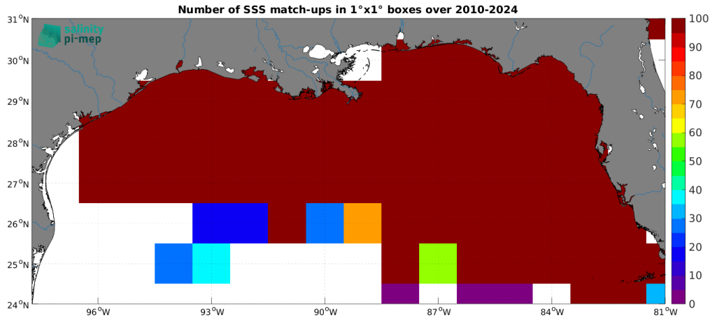
Figure 5: Number of SSS match-ups between TSG (SAMOS) SSS and the SMOS SSS L3 v335 - 10 Days - 25 km (CATDS-CPDC) SSS product for the Mississippi river plume Pi-MEP region over 1^\circ \times 1^\circ boxes and for the full satellite product period.
