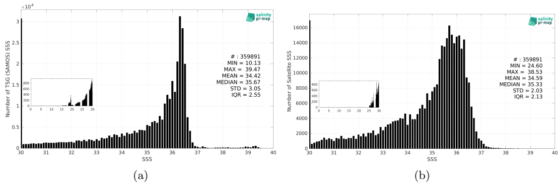
Figure 3: Histograms of SSS from TSG (SAMOS) (a) and SMOS SSS L3 v335 - 10 Days - 25 km (CATDS-CPDC) (b) considering all match-up pairs per bins of 0.1 over the Mississippi river plume Pi-MEP region and for the full satellite product period.
