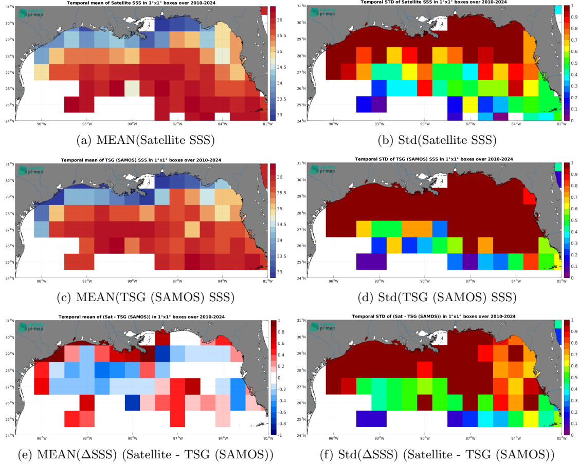
Figure 7: Temporal mean (left) and Std (right) of SSS from SMOS SSS L3 v335 - 10 Days - 25 km (CATDS-CPDC) (top), TSG (SAMOS) (middle), and of \Delta\text{SSS} (Satellite - TSG (SAMOS)). Only match-up pairs are used to generate these maps.
