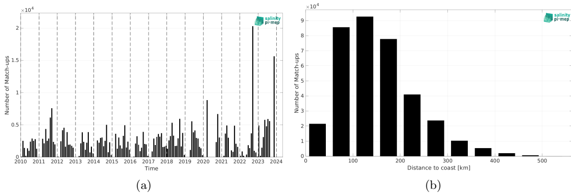
Figure 2: Number of match-ups between TSG (SAMOS) and SMOS SSS L3 v335 - 10 Days - 25 km (CATDS-CPDC) SSS as a function of time (a) and as function of the distance to coast (b) over the Mississippi river plume Pi-MEP region and for the full satellite product period.
