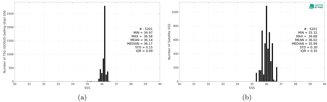
Figure 2: Histograms of SSS from TSG (GOSUD-Sailing-ship) (a) and SMOS SSS L3 v335 - 10 Days - 25 km (CATDS-CPDC) (b) considering all match-up pairs per bins of 0.1 over the Mississippi river plume Pi-MEP region and for the full satellite product period.
