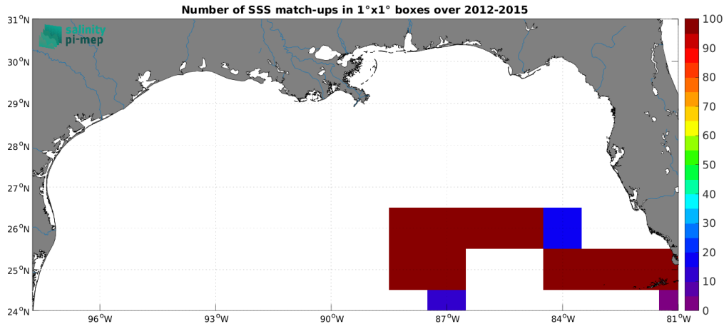
Figure 4: Number of SSS match-ups between TSG (GOSUD-Sailing-ship) SSS and the SMOS SSS L3 v335 - 10 Days - 25 km (CATDS-CPDC) SSS product for the Mississippi river plume Pi-MEP region over 1^\circ \times 1^\circ boxes and for the full satellite product period.
