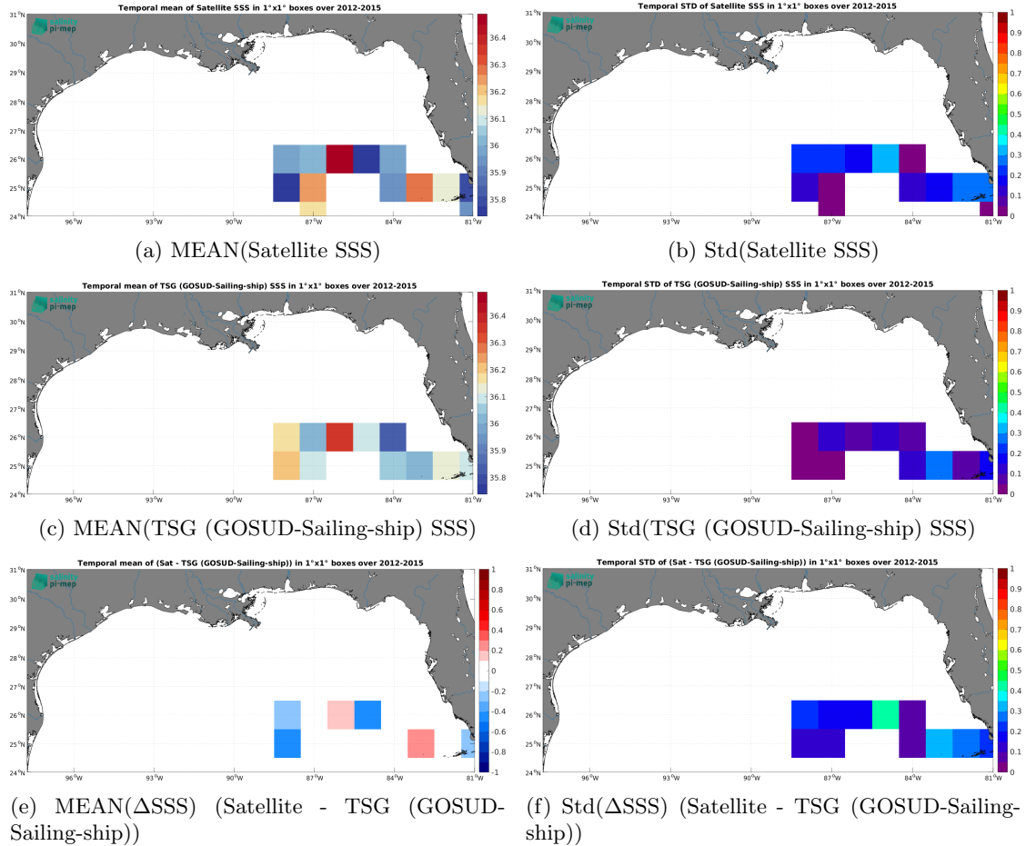
Figure 6: Temporal mean (left) and Std (right) of SSS from SMOS SSS L3 v335 - 10 Days - 25 km (CATDS-CPDC) (top), TSG (GOSUD-Sailing-ship) (middle), and of \Delta\text{SSS} (Satellite - TSG (GOSUD-Sailing-ship)). Only match-up pairs are used to generate these maps.
