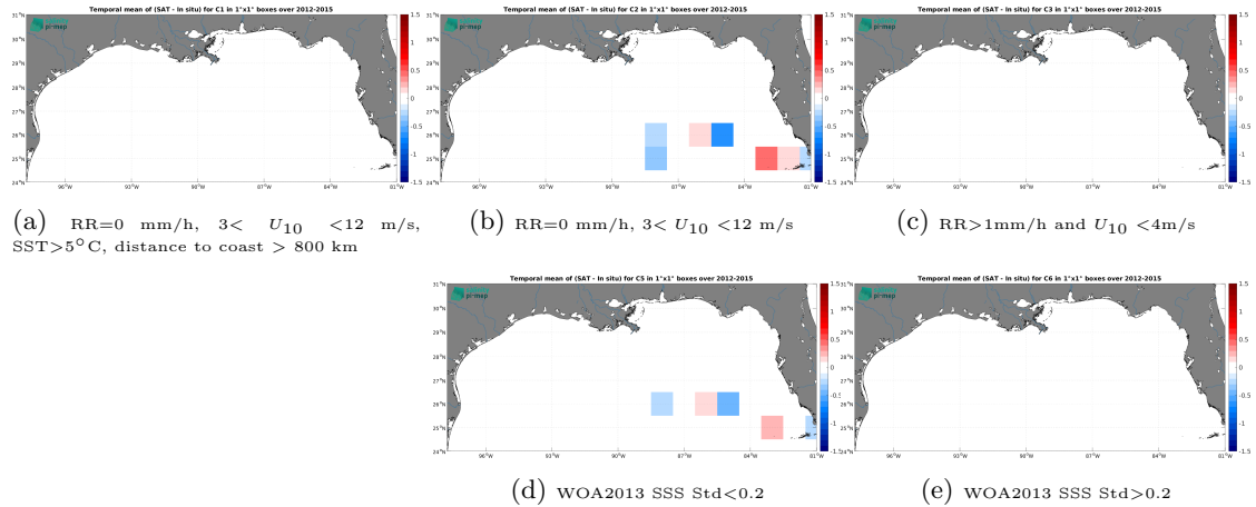
Figure 12: Temporal mean gridded over spatial boxes of size 1^{\circ}\times 1^{\circ} of \Delta SSS (SMOS SSS L3 v335 - 10 Days - 25 km (CATDS-CPDC) - TSG (GOSUD-Sailing-ship)) for 5 different subdatasets corresponding to:RR=0 mm/h, 3 < U_{10} < 12 m/s, SST >5^{\circ}\text{C} , distance to coast > 800 km (a), RR=0 mm/h, 3 < U_{10} < 12 m/s (b), RR >1 mm/h and U_{10} < 4 m/s (c), WOA2013 SSS Std <0.2 (d), WOA2013 SSS Std >0.2 (e).
