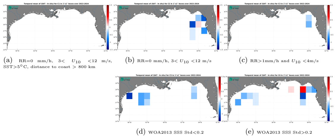
Figure 14: Temporal mean gridded over spatial boxes of size 1^\circ \times 1^\circ of \Delta SSS (SMOS SSS L3 v335 - 10 Days - 25 km (CATDS-CPDC) - Saildrone) for 5 different subdatasets corresponding to: RR=0 mm/h, 3 < U_{10} < 12 m/s, SST > 5°C, distance to coast > 800 km (a), RR=0 mm/h, 3 < U_{10} < 12 m/s (b), RR > 1 mm/h and U_{10} < 4 m/s (c), WOA2013 SSS Std < 0.2 (d), WOA2013 SSS Std > 0.2 (e).
