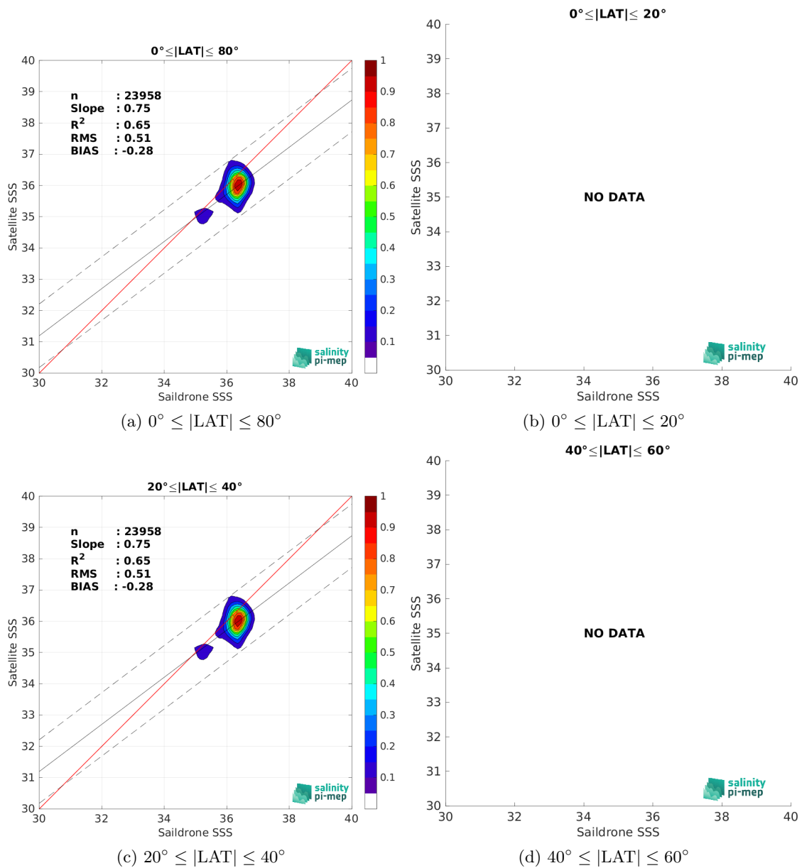
Figure 10: Contour maps of the concentration of SMOS SSS L3 v335 - 10 Days - 25 km (CATDS-CPDC) SSS (y-axis) versus Saildrone SSS (x-axis) at match-up pairs for different latitude bands. For each plot, the red line shows x=y . The black thin and dashed lines indicate a linear fit through the data cloud and the \pm 95\% confidence levels, respectively. The number match-up pairs n , the slope and R^2 coefficient of the linear fit, the root mean square (RMS) and the mean bias between satellite and in situ data are indicated for each latitude band in each plots.
