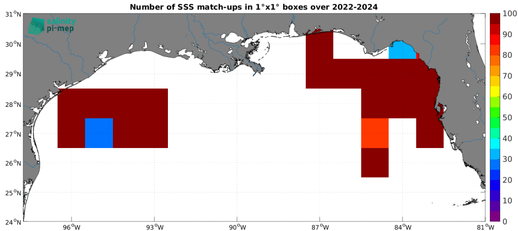
Figure 5: Number of SSS match-ups between Saildrone SSS and the SMOS SSS L3 v335 - 10 Days - 25 km (CATDS-CPDC) SSS product for the Mississippi river plume Pi-MEP region over 1^\circ \times 1^\circ boxes and for the full satellite product period.
