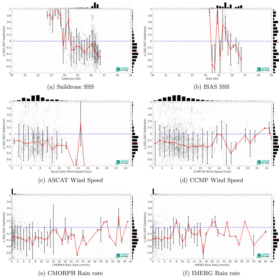
Figure 12: \Delta \text{SSS} (Satellite - Saildrone) sorted as function of SSS values (a), ISAS SSS (b), ASCAT Wind speed (c), CCMP Wind speed (d), CMORPH rain rate (e) and IMERG rain rate (f). In all plots the median and Std of \Delta \text{SSS} for each bin is indicated by the red curves and black vertical thick bars ( \pm 1 \text{ Std} ).
