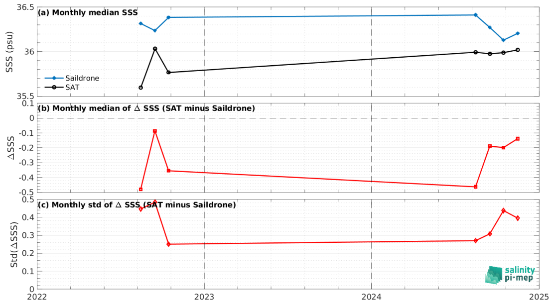
Figure 8: Time series of the monthly median SSS (top), median of \Delta SSS (Satellite - Saildrone) and Std of \Delta SSS (Satellite - Saildrone) over the Mississippi river plume Pi-MEP region considering all match-ups collected by the Pi-MEP.
