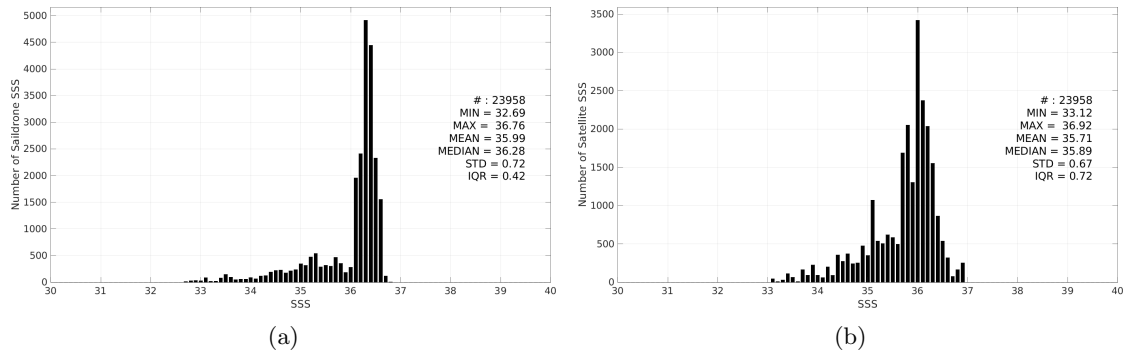
Figure 3: Histograms of SSS from Saildrone (a) and SMOS SSS L3 v335 - 10 Days - 25 km (CATDS-CPDC) (b) considering all match-up pairs per bins of 0.1 over the Mississippi river plume Pi-MEP region and for the full satellite product period.
