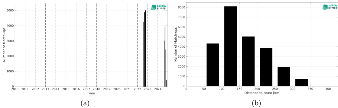
Figure 2: Number of match-ups between Saildrone and SMOS SSS L3 v335 - 10 Days - 25 km (CATDS-CPDC) SSS as a function of time (a) and as function of the distance to coast (b) over the Mississippi river plume Pi-MEP region and for the full satellite product period.
