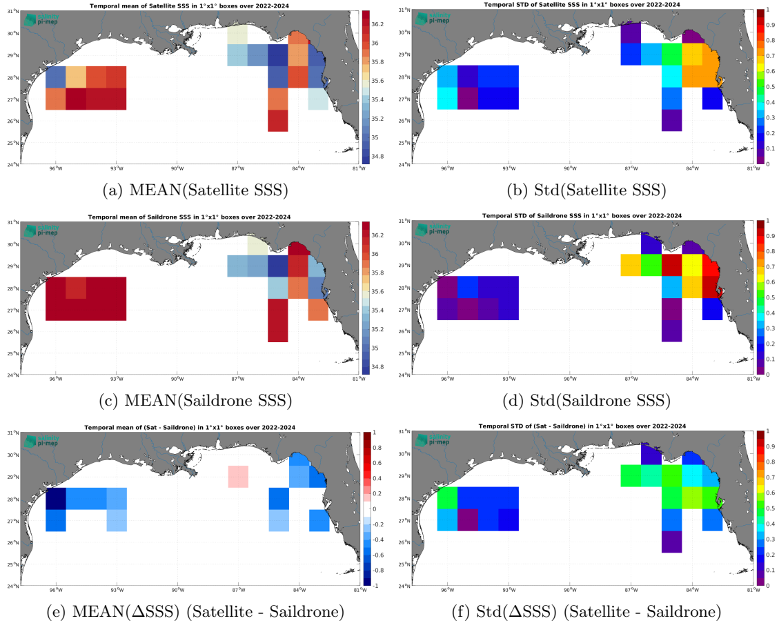
Figure 7: Temporal mean (left) and Std (right) of SSS from SMOS SSS L3 v335 - 10 Days - 25 km (CATDS-CPDC) (top), Sairdrone (middle), and of \Delta SSS (Satellite - Sairdrone). Only match-up pairs are used to generate these maps.
