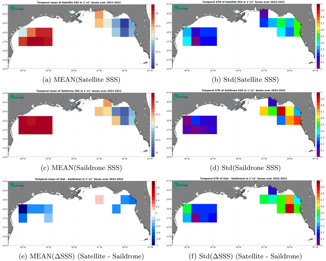
Figure 6: Temporal mean (left) and Std (right) of SSS from SMOS SSS L3 v335 - 10 Days - 25 km (CATDS-CPDC) (top), Sairdrone (middle), and of \Delta SSS (Satellite - Sairdrone). Only match-up pairs are used to generate these maps.
