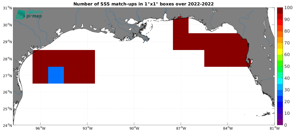
Figure 4: Number of SSS match-ups between Saildrone SSS and the SMOS SSS L3 v335 - 10 Days - 25 km (CATDS-CPDC) SSS product for the Mississippi river plume Pi-MEP region over 1^\circ \times 1^\circ boxes and for the full satellite product period.
