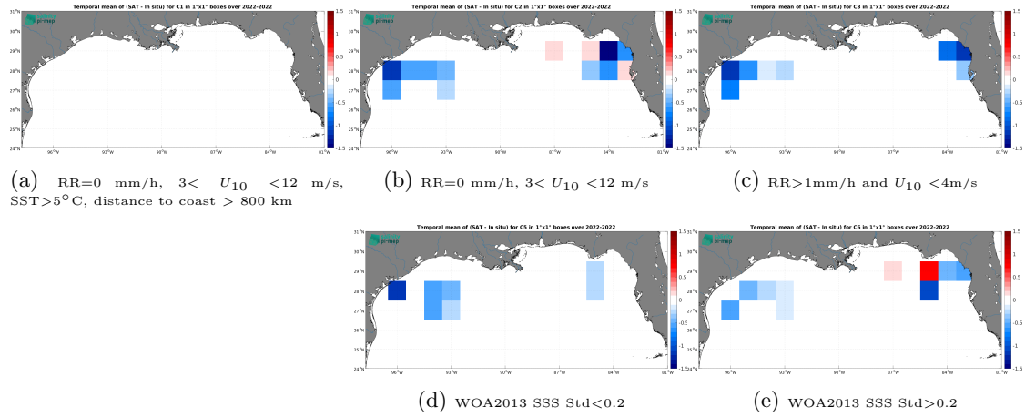
Figure 12: Temporal mean gridded over spatial boxes of size 1^{\circ}\times 1^{\circ} of \Delta\text{SSS} (SMOS SSS L3 v335 - 10 Days - 25 km (CATDS-CPDC) - Saildrone) for 5 different subdatasets corresponding to:RR=0 mm/h, 3 < U_{10} < 12 m/s, SST >5^{\circ}\text{C} , distance to coast > 800 km (a), RR=0 mm/h, 3 < U_{10} < 12 m/s (b), RR >1 mm/h and U_{10} < 4 m/s (c), WOA2013 SSS Std <0.2 (d), WOA2013 SSS Std >0.2 (e).
