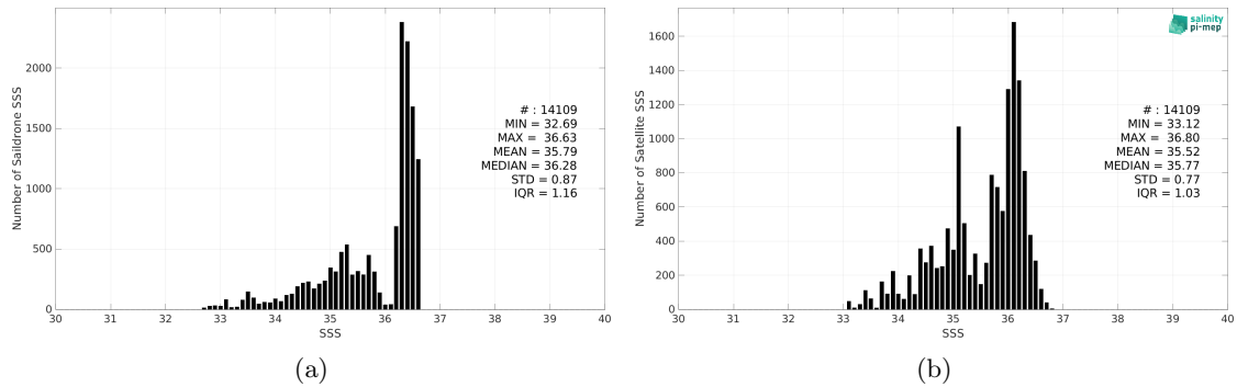
Figure 2: Histograms of SSS from Sairdron (a) and SMOS SSS L3 v335 - 10 Days - 25 km (CATDS-CPDC) (b) considering all match-up pairs per bins of 0.1 over the Mississippi river plume Pi-MEP region and for the full satellite product period.
