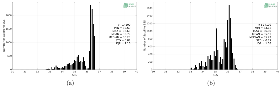
Figure 2: Histograms of SSS from Sairdrone (a) and SMOS SSS L3 v335 - 10 Days - 25 km (CATDS-CPDC) (b) considering all match-up pairs per bins of 0.1 over the Mississippi river plume Pi-MEP region and for the full satellite product period.
