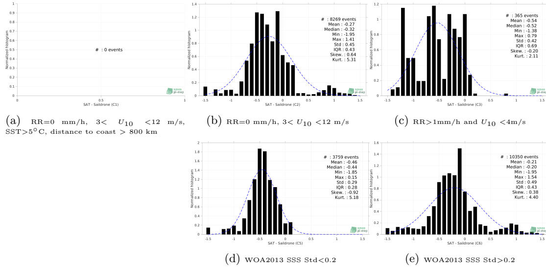
Figure 13: Normalized histogram of \Delta SSS (SMOS SSS L3 v335 - 10 Days - 25 km (CATDS-CPDC) - Salldrone) for 5 different subdatasets corresponding to: RR=0 mm/h, 3 < U_{10} < 12 m/s, SST > 5°C, distance to coast > 800 km (a), RR=0 mm/h, 3 < U_{10} < 12 m/s (b), RR > 1mm/h and U_{10} < 4 m/s (c), WOA2013 SSS Std < 0.2 (d), WOA2013 SSS Std > 0.2 (e).
