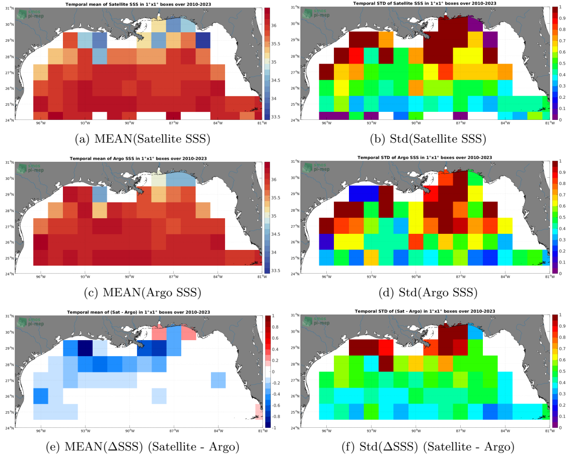
Figure 6: Temporal mean (left) and Std (right) of SSS from SMOS SSS L3 v335 - 10 Days - 25 km (CATDS-CPDC) (top), Argo (middle), and of \Delta\text{SSS} (Satellite - Argo). Only match-up pairs are used to generate these maps.
