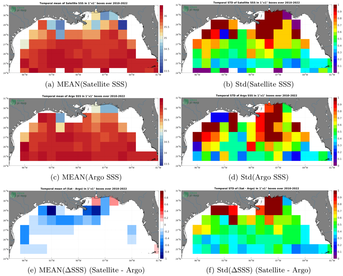
Figure 6: Temporal mean (left) and Std (right) of SSS from SMOS SSS L3 v335 - 10 Days - 25 km (CATDS-CPDC) (top), Argo (middle), and of \Delta SSS (Satellite - Argo). Only match-up pairs are used to generate these maps.
