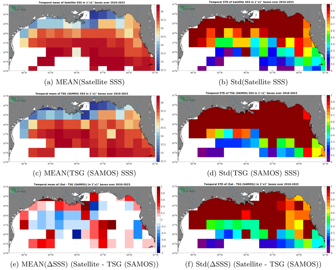
Figure 6: Temporal mean (left) and Std (right) of SSS from SMOS SSS L3 v332 - 9 Days (CATDS-CPDC) (top), TSG (SAMOS) (middle), and of \Delta SSS (Satellite - TSG (SAMOS)). Only match-up pairs are used to generate these maps.
