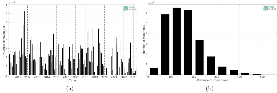
Figure 1: Number of match-ups between TSG (SAMOS) and SMOS SSS L3 v332 - 9 Days (CATDS-CPDC) SSS as a function of time (a) and as function of the distance to coast (b) over the Mississippi river plume Pi-MEP region and for the full satellite product period.
