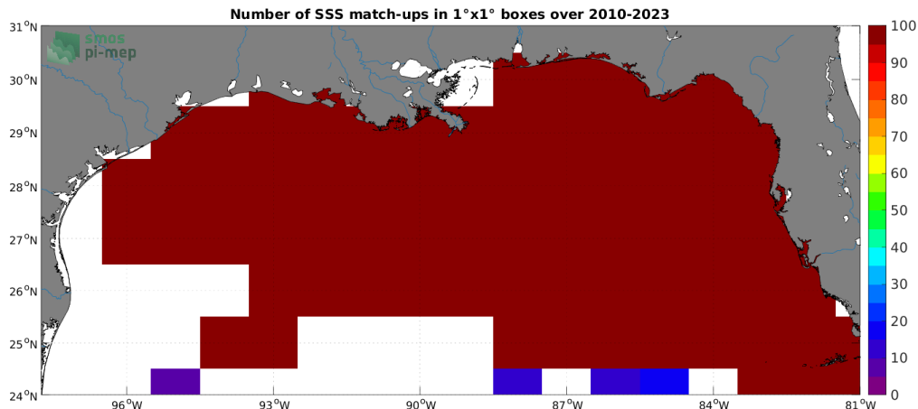
Figure 4: Number of SSS match-ups between TSG (SAMOS) SSS and the SMOS SSS L3 v332 - 9 Days (CATDS-CPDC) SSS product for the Mississippi river plume Pi-MEP region over 1^\circ \times 1^\circ boxes and for the full satellite product period.
