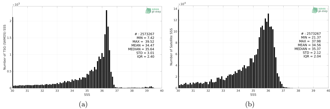
Figure 2: Histograms of SSS from TSG (SAMOS) (a) and SMOS SSS L3 v332 - 9 Days (CATDS-CPDC) (b) considering all match-up pairs per bins of 0.1 over the Mississippi river plume Pi-MEP region and for the full satellite product period.
