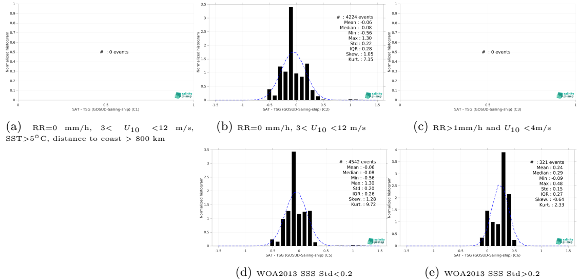
Figure 15: Normalized histogram of \Delta SSS (SMOS SSS L3 v332 - 9 Days (CATDS-CPDC) - TSG (GOSUD-Sailing-ship)) for 5 different subdatasets corresponding to: RR=0 mm/h, 3 < U_{10} < 12 m/s, SST > 5°C, distance to coast > 800 km (a), RR=0 mm/h, 3 < U_{10} < 12 m/s (b), RR > 1mm/h and U_{10} < 4 m/s (c), WOA2013 SSS Std < 0.2 (d), WOA2013 SSS Std > 0.2 (e).
