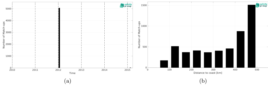
Figure 2: Number of match-ups between TSG (GOSUD-Sailing-ship) and SMOS SSS L3 v332 - 9 Days (CATDS-CPDC) SSS as a function of time (a) and as function of the distance to coast (b) over the Mississippi river plume Pi-MEP region and for the full satellite product period.
