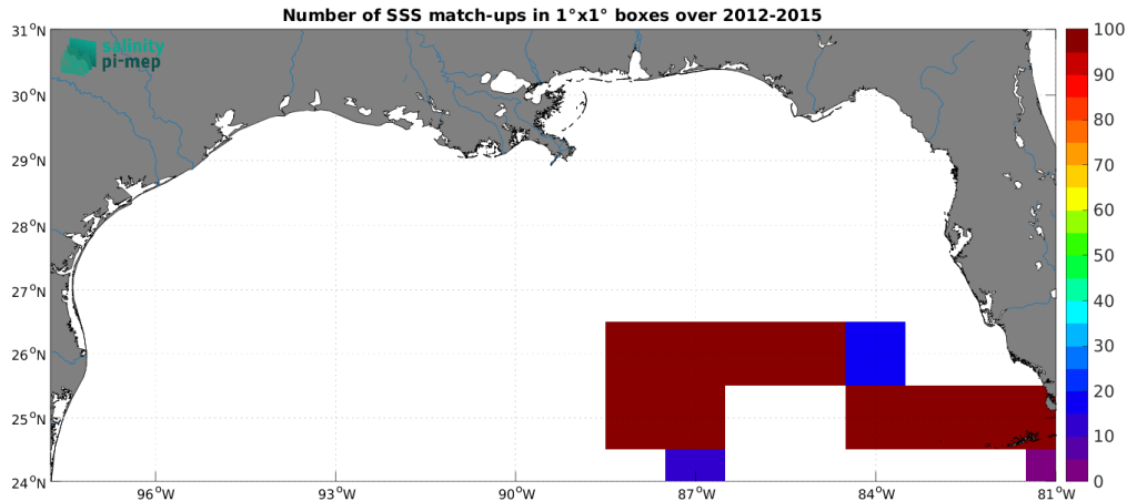
Figure 5: Number of SSS match-ups between TSG (GOSUD-Sailing-ship) SSS and the SMOS SSS L3 v332 - 9 Days (CATDS-CPDC) SSS product for the Mississippi river plume Pi-MEP region over 1^\circ \times 1^\circ boxes and for the full satellite product period.
