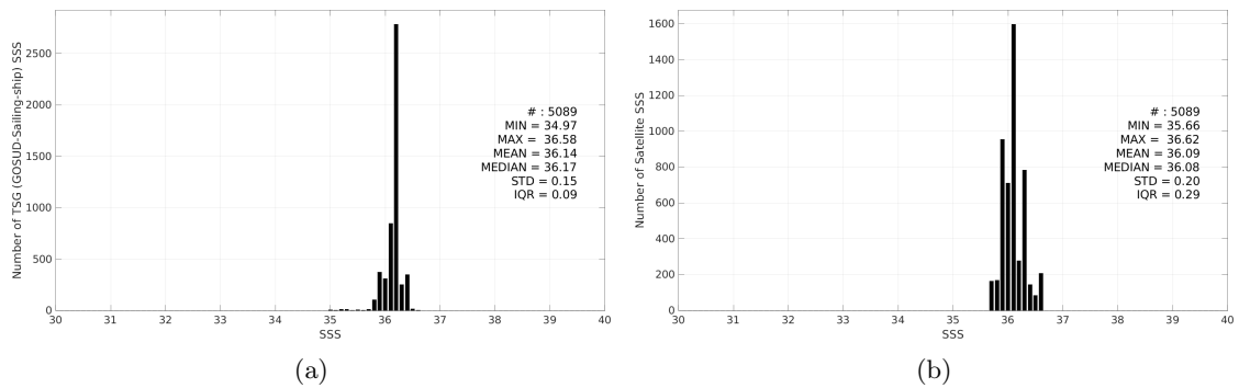
Figure 3: Histograms of SSS from TSG (GOSUD-Sailing-ship) (a) and SMOS SSS L3 v332 - 9 Days (CATDS-CPDC) (b) considering all match-up pairs per bins of 0.1 over the Mississippi river plume Pi-MEP region and for the full satellite product period.
