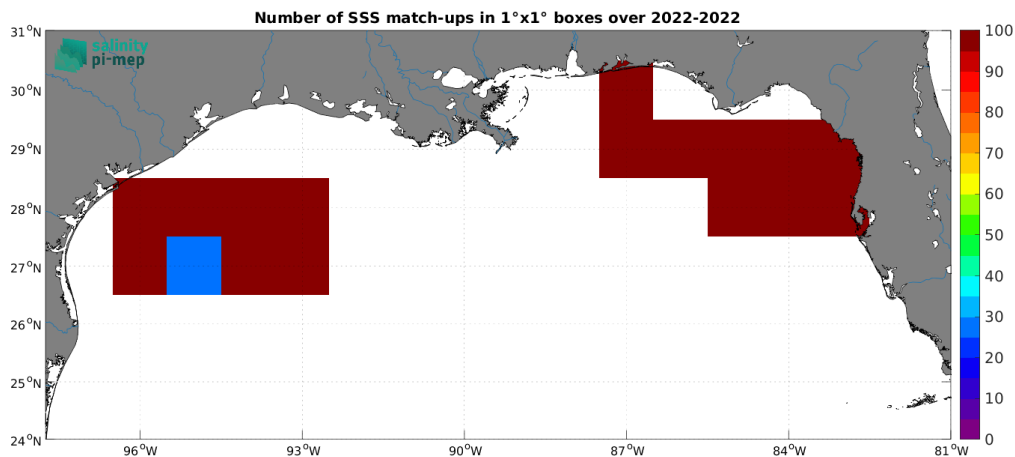
Figure 5: Number of SSS match-ups between Saildrone SSS and the SMOS SSS L3 v332 - 9 Days (CATDS-CPDC) SSS product for the Mississippi river plume Pi-MEP region over 1^\circ \times 1^\circ boxes and for the full satellite product period.
