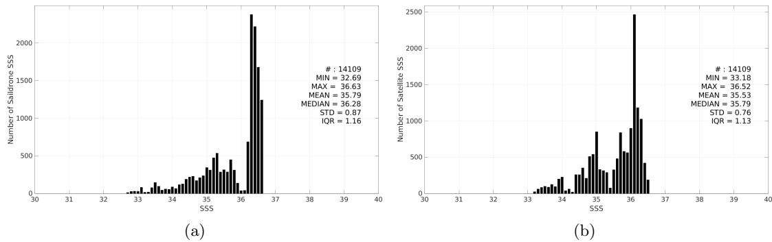
Figure 3: Histograms of SSS from Saildrone (a) and SMOS SSS L3 v332 - 9 Days (CATDS-CPDC) (b) considering all match-up pairs per bins of 0.1 over the Mississippi river plume Pi-MEP region and for the full satellite product period.
