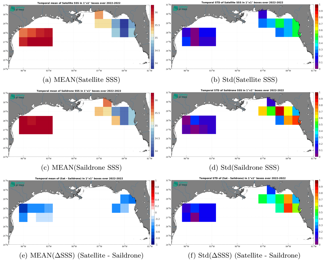
Figure 7: Temporal mean (left) and Std (right) of SSS from SMOS SSS L3 v332 - 9 Days (CATDS-CPDC) (top), Saildrone (middle), and of \Delta SSS (Satellite - Saildrone). Only match-up pairs are used to generate these maps.
