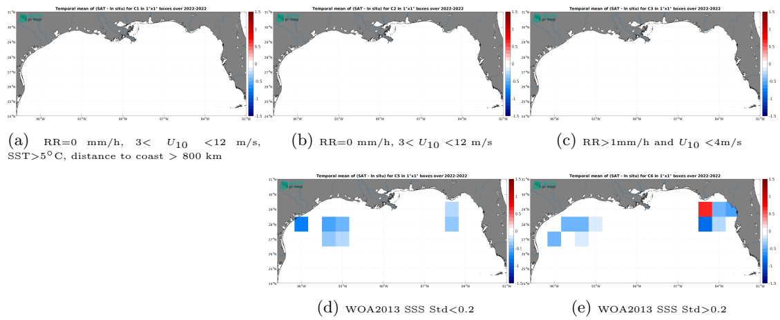
Figure 14: Temporal mean gridded over spatial boxes of size 1^\circ \times 1^\circ of \Delta SSS (SMOS SSS L3 v332 - 9 Days (CATDS-CPDC) - Sairdrone) for 5 different subdatasets corresponding to:RR=0 mm/h, 3 < U_{10} < 12 m/s, SST > 5°C, distance to coast > 800 km (a), RR=0 mm/h, 3 < U_{10} < 12 m/s (b), RR > 1mm/h and U_{10} < 4 m/s (c), WOA2013 SSS Std < 0.2 (d), WOA2013 SSS Std > 0.2 (e).
