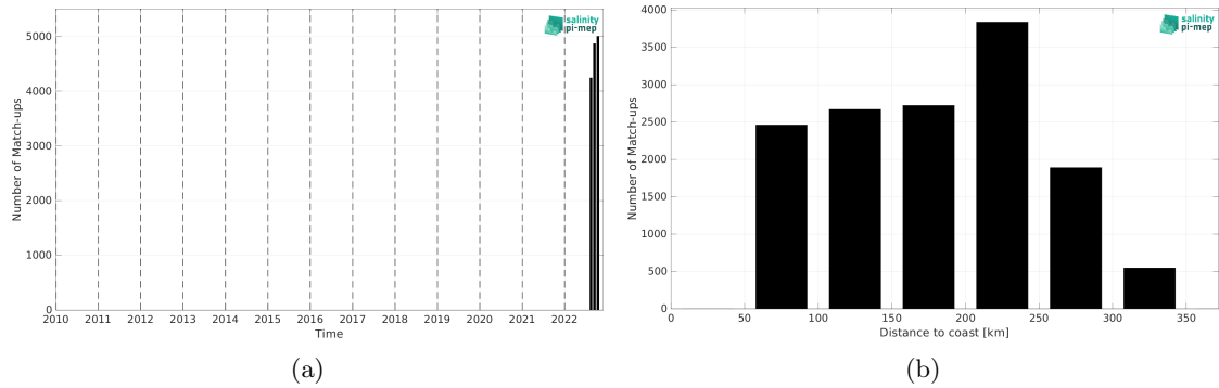
Figure 2: Number of match-ups between Saildrone and SMOS SSS L3 v332 - 9 Days (CATDS-CPDC) SSS as a function of time (a) and as function of the distance to coast (b) over the Mississippi river plume Pi-MEP region and for the full satellite product period.
