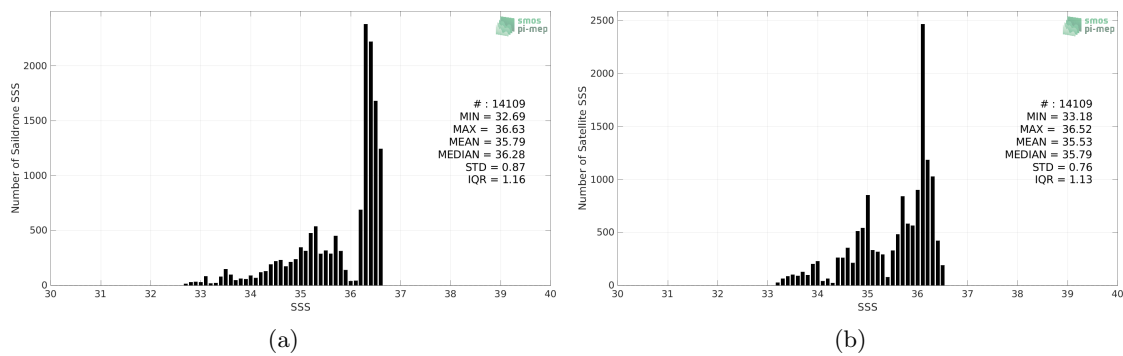
Figure 2: Histograms of SSS from Saildrone (a) and SMOS SSS L3 v332 - 9 Days (CATDS-CPDC) (b) considering all match-up pairs per bins of 0.1 over the Mississippi river plume Pi-MEP region and for the full satellite product period.
