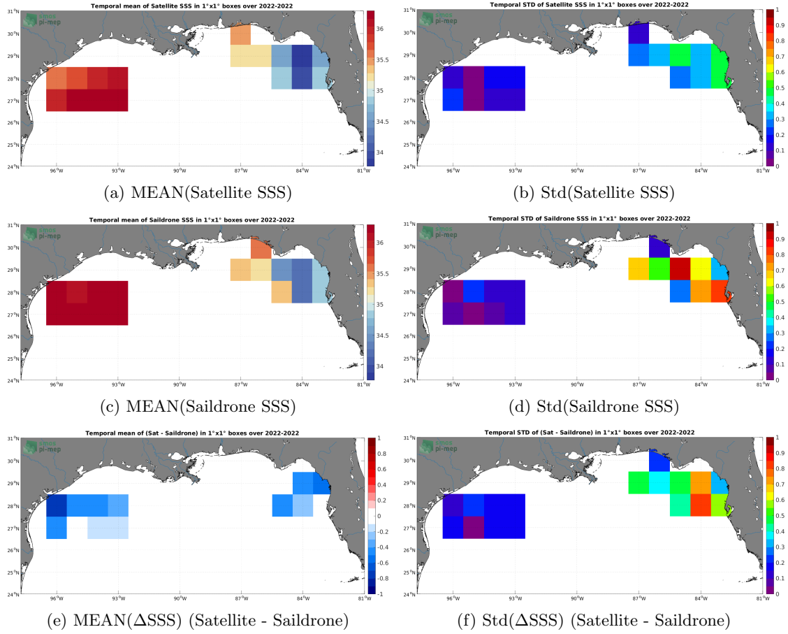
Figure 6: Temporal mean (left) and Std (right) of SSS from SMOS SSS L3 v332 - 9 Days (CATDS-CPDC) (top), Saildrone (middle), and of \Delta SSS (Satellite - Saildrone). Only match-up pairs are used to generate these maps.
