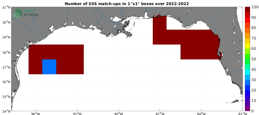
Figure 4: Number of SSS match-ups between Saildrone SSS and the SMOS SSS L3 v332 - 9 Days (CATDS-CPDC) SSS product for the Mississippi river plume Pi-MEP region over 1^\circ \times 1^\circ boxes and for the full satellite product period.
