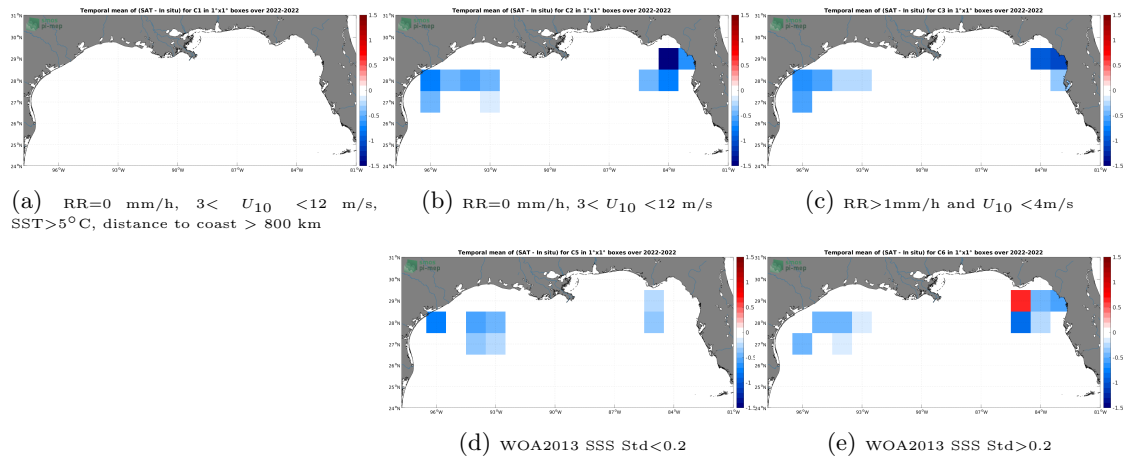
Figure 12: Temporal mean gridded over spatial boxes of size 1^{\circ}\times 1^{\circ} of \Delta\text{SSS} (SMOS SSS L3 v332 - 9 Days (CATDS-CPDC) - Sairdrone) for 5 different subdatasets corresponding to:RR=0 mm/h, 3 < U_{10} < 12 m/s, SST >5^{\circ}\text{C} , distance to coast > 800 km (a), RR=0 mm/h, 3 < U_{10} < 12 m/s (b), RR >1 mm/h and U_{10} < 4 m/s (c), WOA2013 SSS Std <0.2 (d), WOA2013 SSS Std >0.2 (e).
