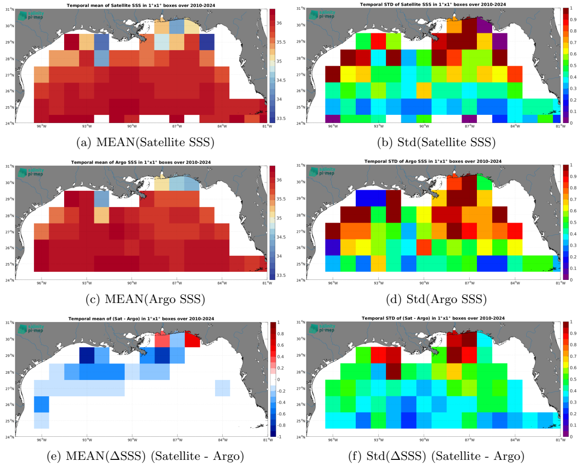
Figure 7: Temporal mean (left) and Std (right) of SSS from SMOS SSS L3 v332 - 9 Days (CATDS-CPDC) (top), Argo (middle), and of \Delta SSS (Satellite - Argo). Only match-up pairs are used to generate these maps.
