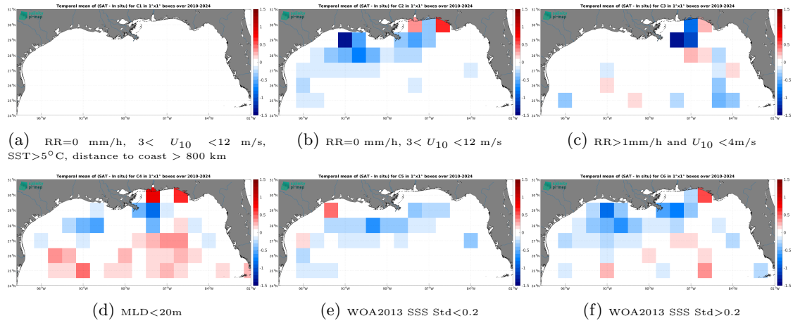
Figure 14: Temporal mean gridded over spatial boxes of size 1^\circ \times 1^\circ of \Delta SSS (SMOS SSS L3 v332 - 9 Days (CATDS-CPDC) - Argo) for 6 different subdatasets corresponding to:RR=0 mm/h, 3 < U_{10} < 12 m/s, SST>5°C, distance to coast > 800 km (a), RR=0 mm/h, 3 < U_{10} < 12 m/s (b), RR>1mm/h and U_{10} < 4 m/s (c),MLD<20m (d),WOA2013 SSS Std<0.2 (e),WOA2013 SSS Std>0.2 (f).
