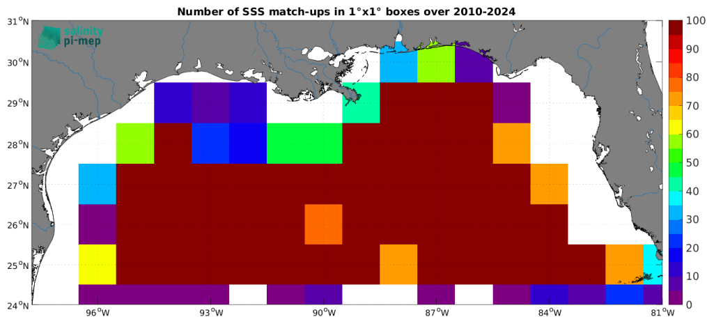
Figure 5: Number of SSS match-ups between Argo SSS and the SMOS SSS L3 v332 - 9 Days (CATDS-CPDC) SSS product for the Mississippi river plume Pi-MEP region over 1^\circ \times 1^\circ boxes and for the full satellite product period.
