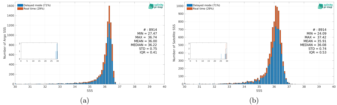
Figure 3: Histograms of SSS from Argo (a) and SMOS SSS L3 v332 - 9 Days (CATDS-CPDC) (b) considering all match-up pairs per bins of 0.1 over the Mississippi river plume Pi-MEP region and for the full satellite product period.
