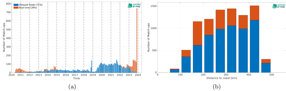
Figure 2: Number of match-ups between Argo and SMOS SSS L3 v332 - 9 Days (CATDS-CPDC) SSS as a function of time (a) and as function of the distance to coast (b) over the Mississippi river plume Pi-MEP region and for the full satellite product period.
