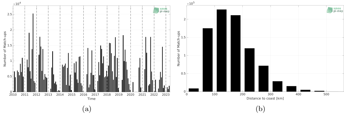
Figure 1: Number of match-ups between TSG (SAMOS) and SMOS SSS L2Q v331 - 0.25 Deg (CATDS-CPDC) SSS as a function of time (a) and as function of the distance to coast (b) over the Mississippi river plume Pi-MEP region and for the full satellite product period.
