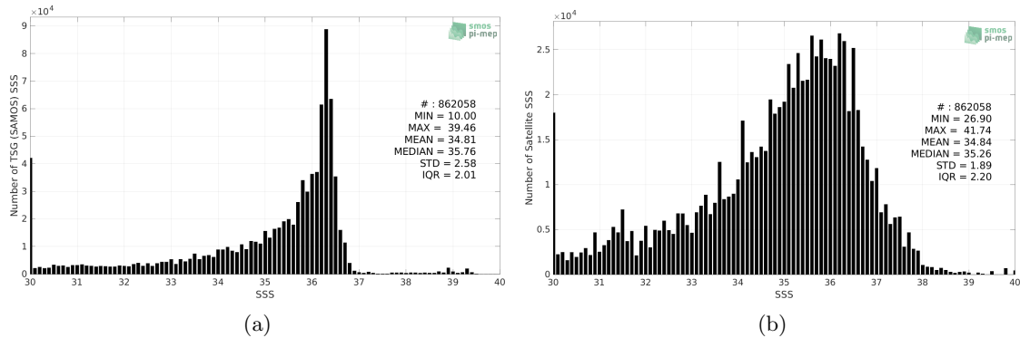
Figure 2: Histograms of SSS from TSG (SAMOS) (a) and SMOS SSS L2Q v331 - 0.25 Deg (CATDS-CPDC) (b) considering all match-up pairs per bins of 0.1 over the Mississippi river plume Pi-MEP region and for the full satellite product period.
