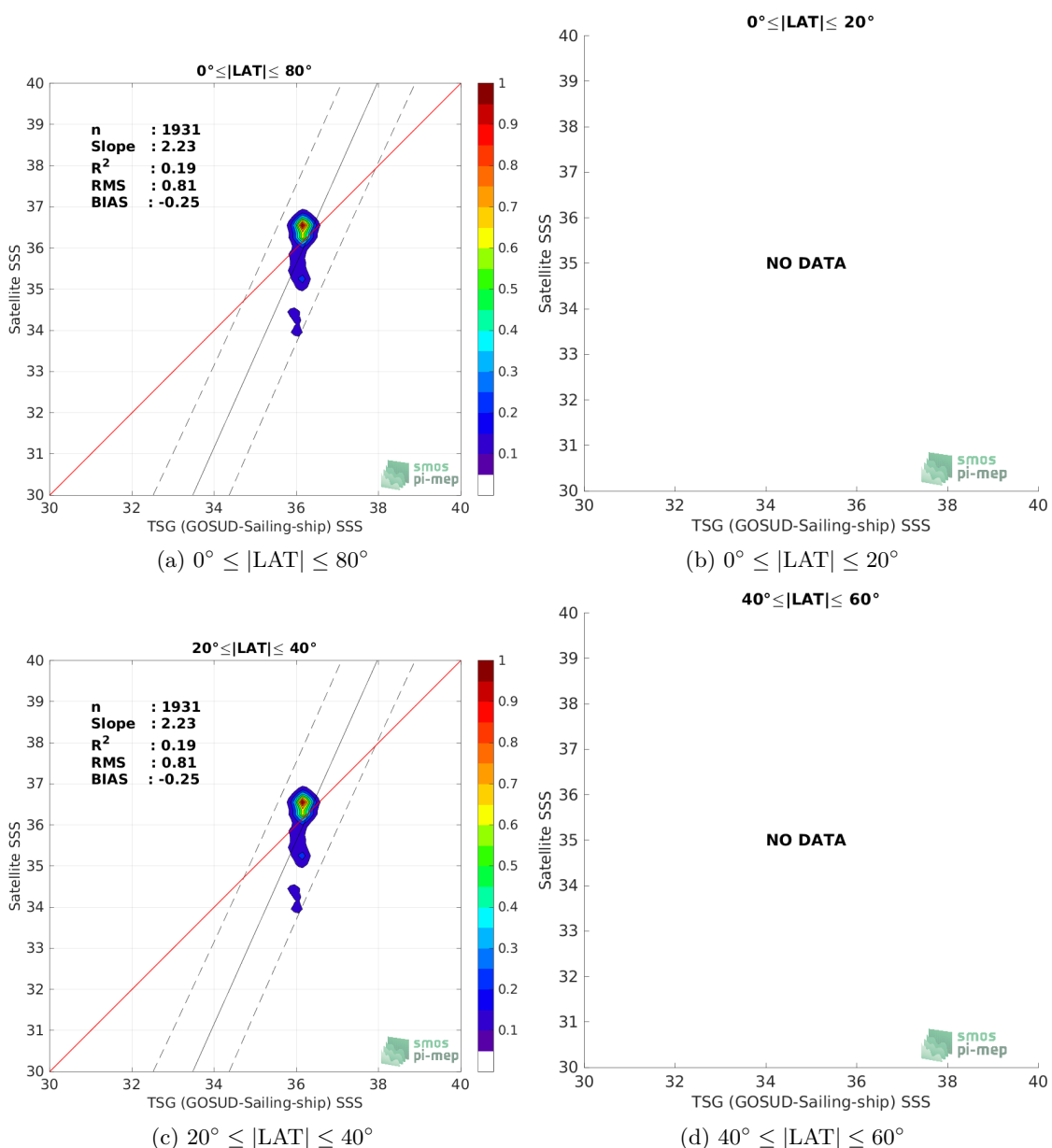
Figure 9: Contour maps of the concentration of SMOS SSS L2Q v331 - 0.25 Deg (CATDS-CPDC) SSS (y-axis) versus TSG (GOSUD-Sailing-ship) SSS (x-axis) at match-up pairs for different latitude bands. For each plot, the red line shows x=y . The black thin and dashed lines indicate a linear fit through the data cloud and the \pm 95\% confidence levels, respectively. The number match-up pairs n , the slope and R^2 coefficient of the linear fit, the root mean square (RMS) and the mean bias between satellite and in situ data are indicated for each latitude band in each plots.
