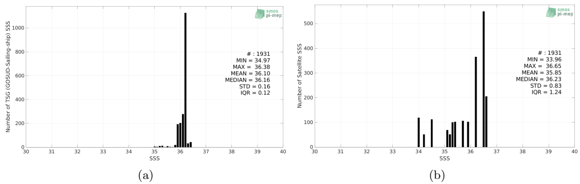
Figure 2: Histograms of SSS from TSG (GOSUD-Sailing-ship) (a) and SMOS SSS L2Q v331 - 0.25 Deg (CATDS-CPDC) (b) considering all match-up pairs per bins of 0.1 over the Mississippi river plume Pi-MEP region and for the full satellite product period.
