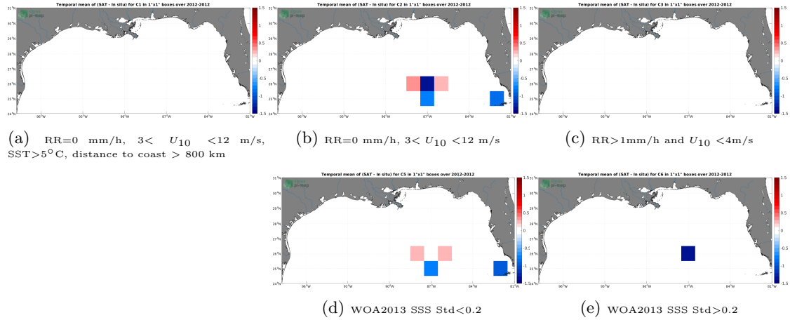
Figure 12: Temporal mean gridded over spatial boxes of size 1^{\circ}\times 1^{\circ} of \Delta SSS (SMOS SSS L2Q v331 - 0.25 Deg (CATDS-CPDC) - TSG (GOSUD-Sailing-ship)) for 5 different subdatasets corresponding to:RR=0 mm/h, 3 < U_{10} < 12 m/s, SST >5^{\circ}\text{C} , distance to coast > 800 km (a), RR=0 mm/h, 3 < U_{10} < 12 m/s (b), RR >1 mm/h and U_{10} < 4 m/s (c), WOA2013 SSS Std <0.2 (d), WOA2013 SSS Std >0.2 (e).
