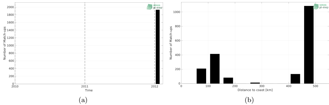
Figure 1: Number of match-ups between TSG (GOSUD-Sailing-ship) and SMOS SSS L2Q v331 - 0.25 Deg (CATDS-CPDC) SSS as a function of time (a) and as function of the distance to coast (b) over the Mississippi river plume Pi-MEP region and for the full satellite product period.
