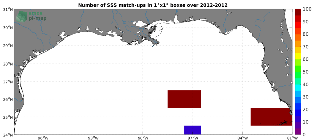
Figure 4: Number of SSS match-ups between TSG (GOSUD-Sailing-ship) SSS and the SMOS SSS L2Q v331 - 0.25 Deg (CATDS-CPDC) SSS product for the Mississippi river plume Pi-MEP region over 1^\circ \times 1^\circ boxes and for the full satellite product period.
