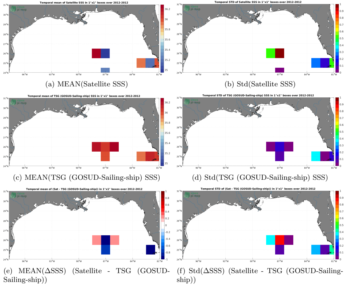
Figure 6: Temporal mean (left) and Std (right) of SSS from SMOS SSS L2Q v331 - 0.25 Deg (CATDS-CPDC) (top), TSG (GOSUD-Sailing-ship) (middle), and of \Delta SSS (Satellite - TSG (GOSUD-Sailing-ship)). Only match-up pairs are used to generate these maps.
