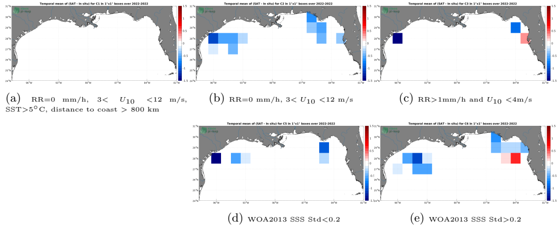
Figure 12: Temporal mean gridded over spatial boxes of size 1^{\circ}\times 1^{\circ} of \Delta\text{SSS} (SMOS SSS L2Q v331 - 0.25 Deg (CATDS-CPDC) - Saildrone) for 5 different subdatasets corresponding to:RR=0 mm/h, 3 < U_{10} < 12 m/s, SST >5^{\circ}\text{C} , distance to coast > 800 km (a), RR=0 mm/h, 3 < U_{10} < 12 m/s (b), RR >1 mm/h and U_{10} < 4 m/s (c), WOA2013 SSS Std <0.2 (d), WOA2013 SSS Std >0.2 (e).
