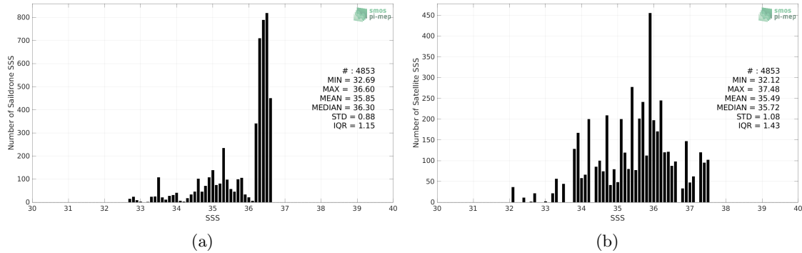
Figure 2: Histograms of SSS from Saildrone (a) and SMOS SSS L2Q v331 - 0.25 Deg (CATDS-CPDC) (b) considering all match-up pairs per bins of 0.1 over the Mississippi river plume Pi-MEP region and for the full satellite product period.
