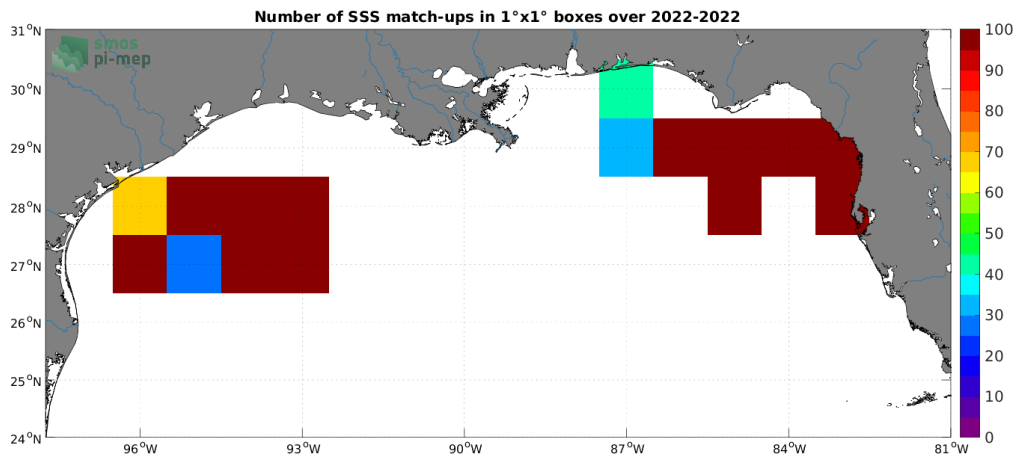
Figure 4: Number of SSS match-ups between Saildrone SSS and the SMOS SSS L2Q v331 - 0.25 Deg (CATDS-CPDC) SSS product for the Mississippi river plume Pi-MEP region over 1^\circ \times 1^\circ boxes and for the full satellite product period.
