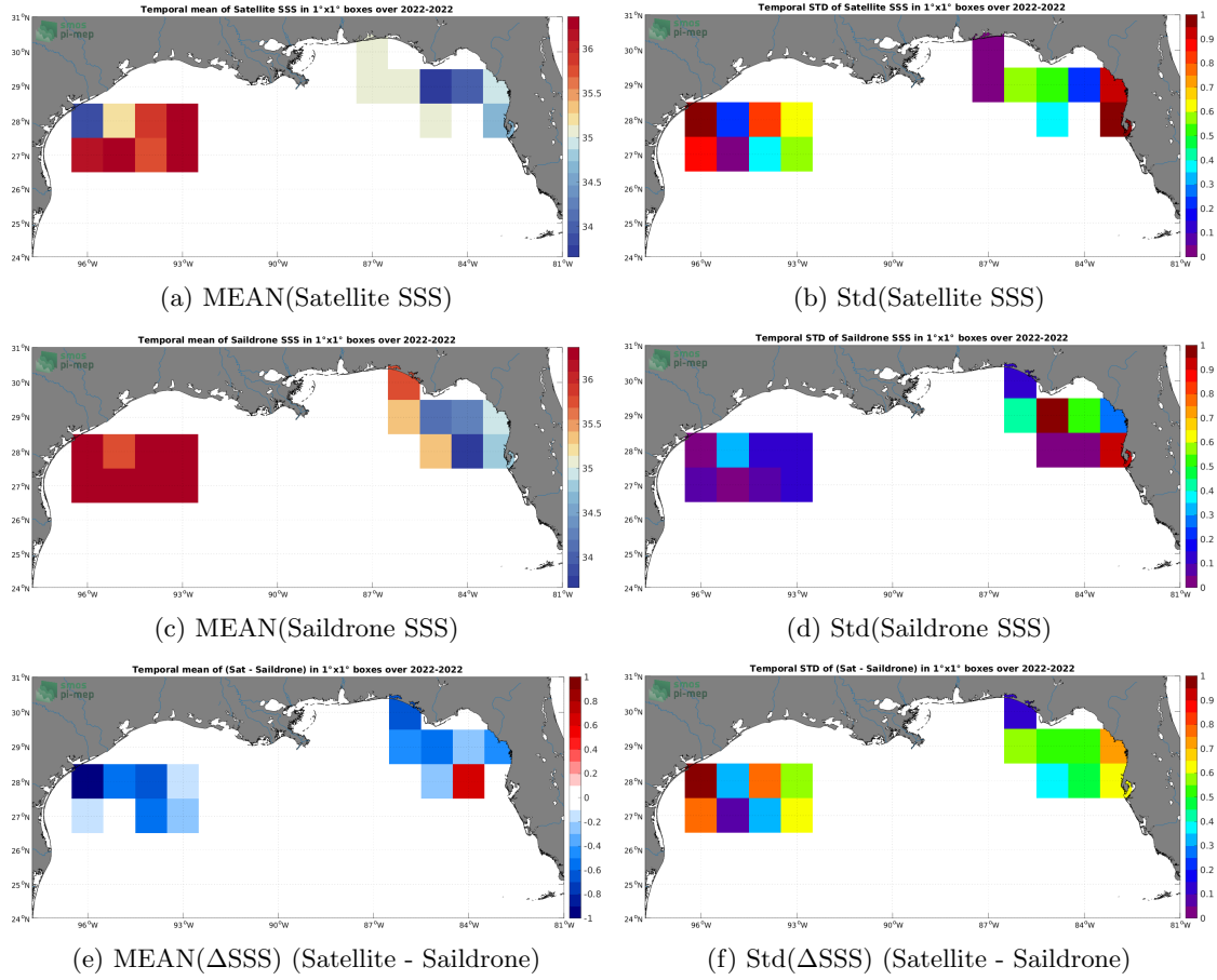
Figure 6: Temporal mean (left) and Std (right) of SSS from SMOS SSS L2Q v331 - 0.25 Deg (CATDS-CPDC) (top), Saildrone (middle), and of \Delta SSS (Satellite - Saildrone). Only match-up pairs are used to generate these maps.
