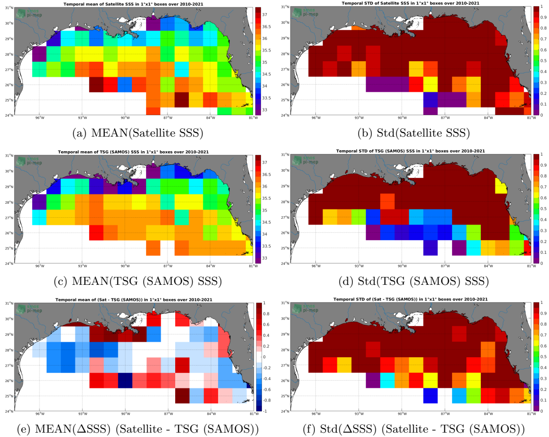
Figure 6: Temporal mean (left) and Std (right) of SSS from SMOS SSS L2Q v321 - 0.25 Deg (CATDS-CPDC) (top), TSG (SAMOS) (middle), and of \Delta\text{SSS} (Satellite - TSG (SAMOS)). Only match-up pairs are used to generate these maps.
