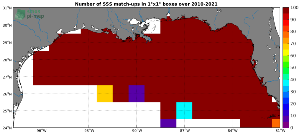
Figure 4: Number of SSS match-ups between TSG (SAMOS) SSS and the SMOS SSS L2Q v321 - 0.25 Deg (CATDS-CPDC) SSS product for the Mississippi river plume Pi-MEP region over 1^\circ \times 1^\circ boxes and for the full satellite product period.
