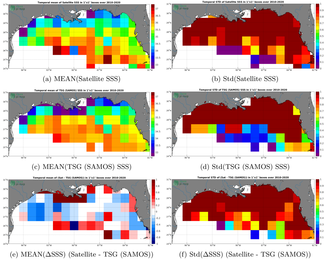
Figure 6: Temporal mean (left) and Std (right) of SSS from SMOS SSS L2Q v321 - 0.25 Deg (CATDS-CPDC) (top), TSG (SAMOS) (middle), and of \Delta SSS (Satellite - TSG (SAMOS)). Only match-up pairs are used to generate these maps.
