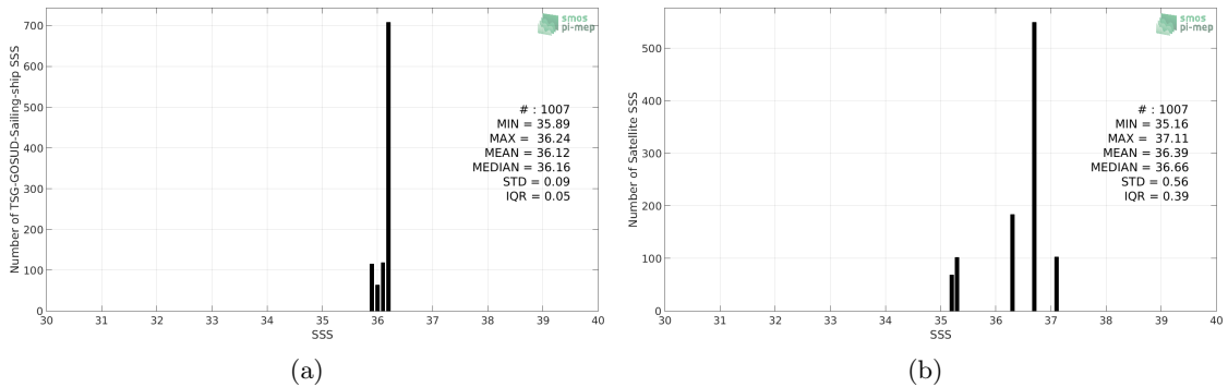
Figure 2: Histograms of SSS from TSG-GOSUD-Sailing-ship (a) and SMOS L2Q v321 - 0.25 Deg (CATDS-CPDC) (b) considering all match-up pairs per bins of 0.1 over the Mississippi river plume Pi-MEP region and for the full satellite product period.
