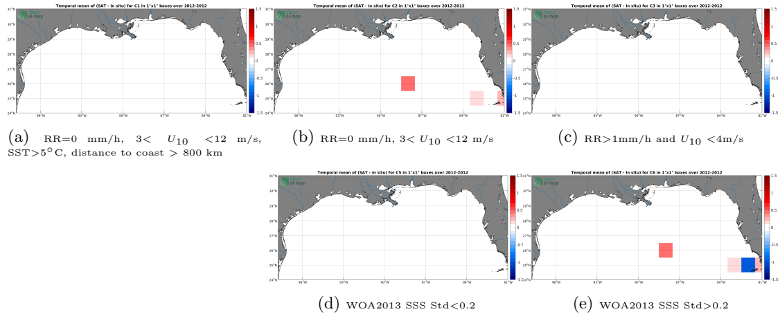
Figure 12: Temporal mean gridded over spatial boxes of size 1^{\circ}\times 1^{\circ} of \Delta SSS (SMOS L2Q v321 - 0.25 Deg (CATDS-CPDC) - TSG-GOSUD-Sailing-ship) for 5 different subdatasets corresponding to:RR=0 mm/h, 3 < U_{10} < 12 m/s, SST >5^{\circ}\text{C} , distance to coast > 800 km (a), RR=0 mm/h, 3 < U_{10} < 12 m/s (b), RR >1 mm/h and U_{10} < 4 m/s (c), WOA2013 SSS Std <0.2 (d), WOA2013 SSS Std >0.2 (e).
