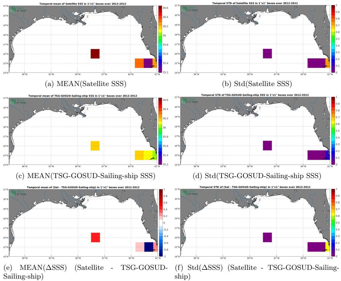
Figure 6: Temporal mean (left) and Std (right) of SSS from SMOS L2Q v321 - 0.25 Deg (CATDS-CPDC) (top), TSG-GOSUD-Sailing-ship (middle), and of \Delta SSS (Satellite - TSG-GOSUD-Sailing-ship). Only match-up pairs are used to generate these maps.
