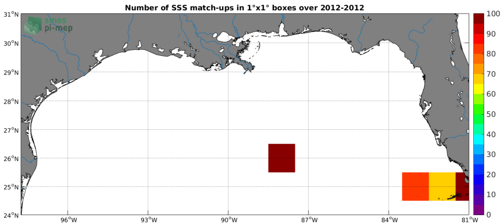
Figure 4: Number of SSS match-ups between TSG-GOSUD-Sailing-ship SSS and the SMOS L2Q v321 - 0.25 Deg (CATDS-CPDC) SSS product for the Mississippi river plume Pi-MEP region over 1°x1° boxes and for the full satellite product period.
