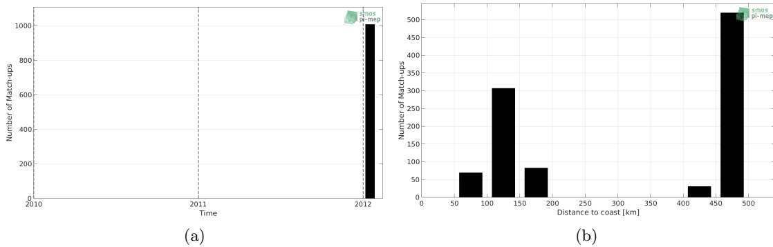
Figure 1: Number of match-ups between TSG-GOSUD-Sailing-ship and SMOS L2Q v321 - 0.25 Deg (CATDS-CPDC) SSS as a function of time (a) and as function of the distance to coast (b) over the Mississippi river plume Pi-MEP region and for the full satellite product period.
