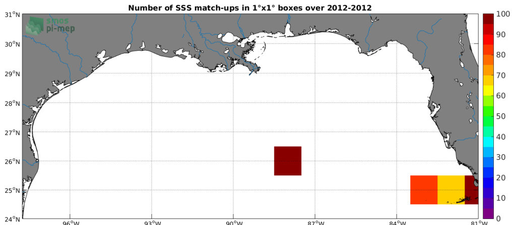
Figure 4: Number of SSS match-ups between TSG-GOSUD-Sailing-ship SSS and the SMOS-L3-CATDS-CPDC-V321-L2Q SSS product for the Mississippi river plume Pi-MEP region over 1^\circ \times 1^\circ boxes and for the full satellite product period.
