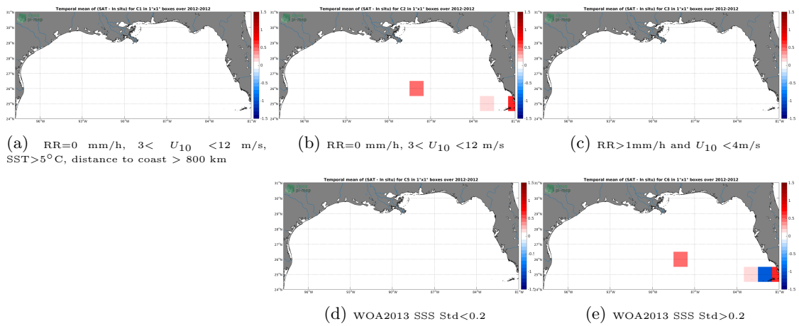
Figure 12: Temporal mean gridded over spatial boxes of size 1^\circ \times 1^\circ of \Delta SSS (SMOS-L3-CATDS-CPDC-V321-L2Q - TSG-GOSUD-Sailing-ship) for 5 different subdatasets corresponding to: RR=0 mm/h, 3 < U_{10} < 12 m/s, SST > 5°C, distance to coast > 800 km (a), RR=0 mm/h, 3 < U_{10} < 12 m/s (b), RR > 1mm/h and U_{10} < 4 m/s (c), WOA2013 SSS Std < 0.2 (d), WOA2013 SSS Std > 0.2 (e).
