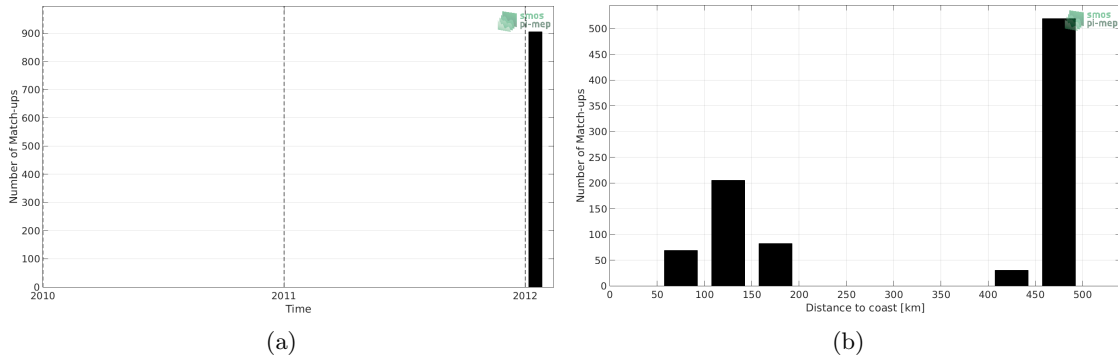
Figure 1: Number of match-ups between TSG-GOSUD-Sailing-ship and SMOS-L3-CATDS-CPDC-V321-L2Q SSS as a function of time (a) and as function of the distance to coast (b) over the Mississippi river plume Pi-MEP region and for the full satellite product period.
