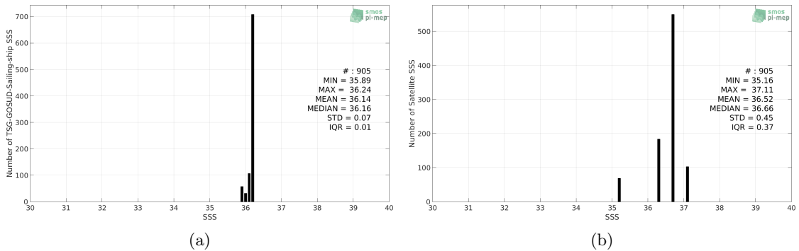
Figure 2: Histograms of SSS from TSG-GOSUD-Sailing-ship (a) and SMOS-L3-CATDS-CPDC-V321-L2Q (b) considering all match-up pairs per bins of 0.1 over the Mississippi river plume Pi-MEP region and for the full satellite product period.
