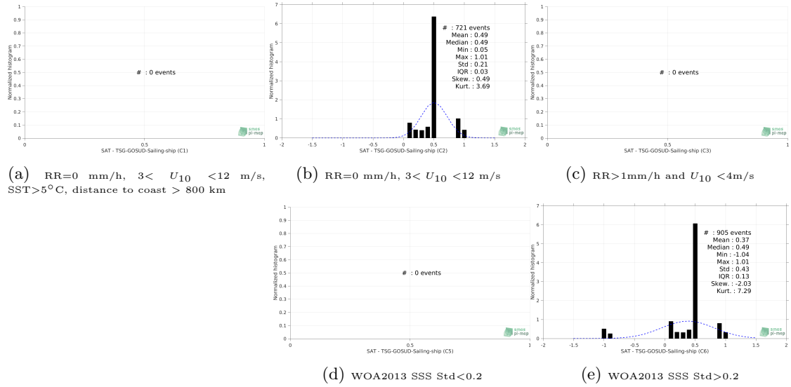
Figure 13: Normalized histogram of \Delta\text{SSS} (SMOS-L3-CATDS-CPDC-V321-L2Q - TSG-GOSUD-Sailing-ship) for 5 different subdatasets corresponding to: RR=0 mm/h, 3 < U_{10} < 12 m/s, SST > 5^\circ\text{C} , distance to coast > 800 km (a), RR=0 mm/h, 3 < U_{10} < 12 m/s (b), RR > 1\text{mm/h} and U_{10} < 4\text{m/s} (c), WOA2013 SSS Std < 0.2 (d), WOA2013 SSS Std > 0.2 (e).
