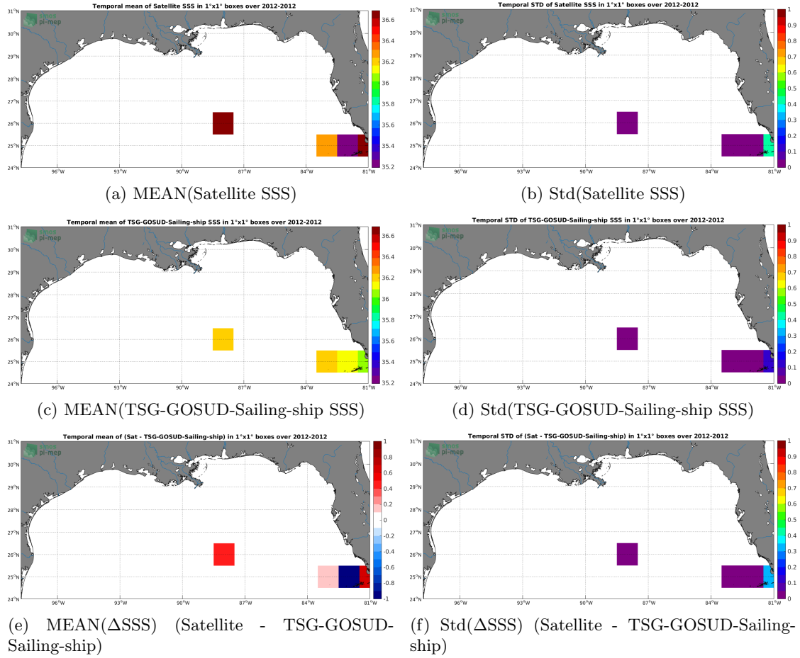
Figure 6: Temporal mean (left) and Std (right) of SSS from SMOS-L3-CATDS-CPDC-V321-L2Q (top), TSG-GOSUD-Sailing-ship (middle), and of \Delta SSS (Satellite - TSG-GOSUD-Sailing-ship). Only match-up pairs are used to generate these maps.
