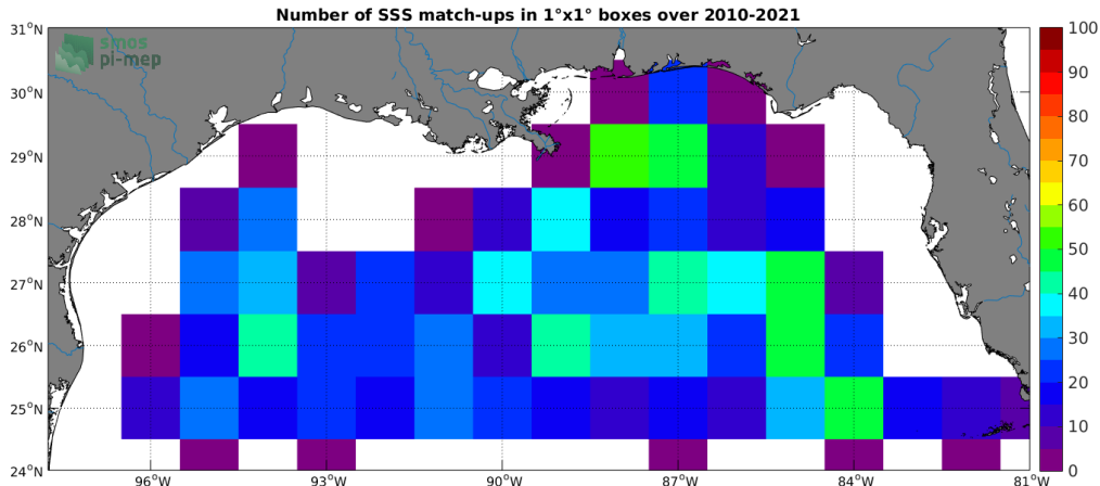
Figure 4: Number of SSS match-ups between Argo SSS and the SMOS SSS L2Q v321 - 0.25 Deg (CATDS-CPDC) SSS product for the Mississippi river plume Pi-MEP region over 1°x1° boxes and for the full satellite product period.
