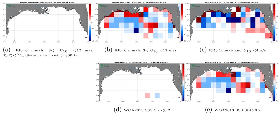
Figure 12: Temporal mean gridded over spatial boxes of size 1^{\circ}\times 1^{\circ} of \Delta\text{SSS} (SMOS L3 v317 - Monthly - 25 km (CATDS-CPDC) - TSG-SAMOS) for 5 different subdatasets corresponding to:RR=0 mm/h, 3 < U_{10} < 12 m/s, SST >5^{\circ}\text{C} , distance to coast > 800 km (a), RR=0 mm/h, 3 < U_{10} < 12 m/s (b), RR >1 mm/h and U_{10} < 4 m/s (c), WOA2013 SSS Std <0.2 (d), WOA2013 SSS Std >0.2 (e).
