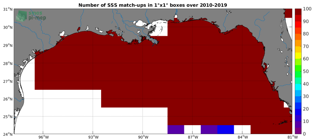
Figure 4: Number of SSS match-ups between TSG-SAMOS SSS and the SMOS L3 v317 - Monthly - 25 km (CATDS-CPDC) SSS product for the Mississippi river plume Pi-MEP region over 1°x1° boxes and for the full satellite product period.
