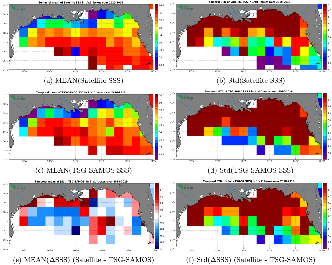
Figure 6: Temporal mean (left) and Std (right) of SSS from SMOS L3 v317 - Monthly - 25 km (CATDS-CPDC) (top), TSG-SAMOS (middle), and of \Delta SSS (Satellite - TSG-SAMOS). Only match-up pairs are used to generate these maps.
