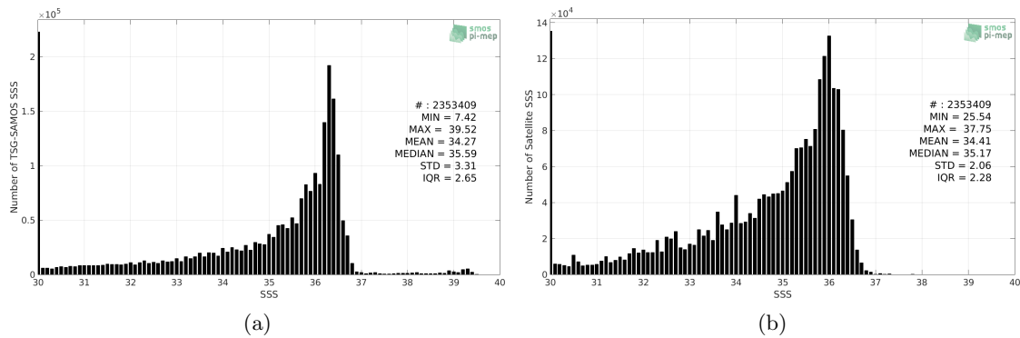
Figure 2: Histograms of SSS from TSG-SAMOS (a) and SMOS L3 v317 - Monthly - 25 km (CATDS-CPDC) (b) considering all match-up pairs per bins of 0.1 over the Mississippi river plume Pi-MEP region and for the full satellite product period.
