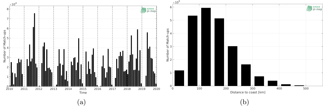
Figure 1: Number of match-ups between TSG-SAMOS and SMOS L3 v317 - Monthly - 25 km (CATDS-CPDC) SSS as a function of time (a) and as function of the distance to coast (b) over the Mississippi river plume Pi-MEP region and for the full satellite product period.
