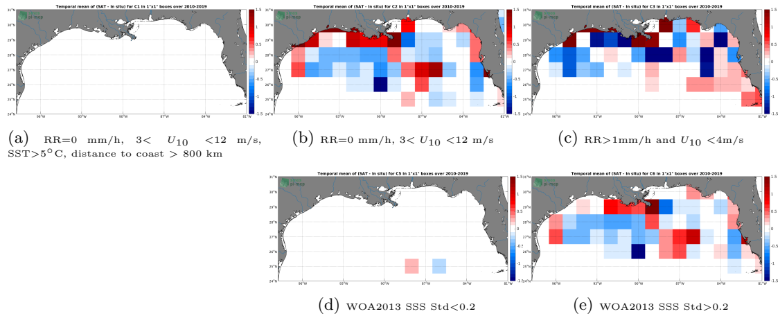
Figure 12: Temporal mean gridded over spatial boxes of size 1^\circ \times 1^\circ of \Delta SSS (SMOS-L3-CATDS-CPDC-V317-MONTHLY-25KM - TSG-SAMOS) for 5 different subdatasets corresponding to: RR=0 mm/h, 3 < U_{10} < 12 m/s, SST > 5^\circ C , distance to coast > 800 km (a), RR=0 mm/h, 3 < U_{10} < 12 m/s (b), RR > 1 mm/h and U_{10} < 4 m/s (c), WOA2013 SSS Std < 0.2 (d), WOA2013 SSS Std > 0.2 (e).
