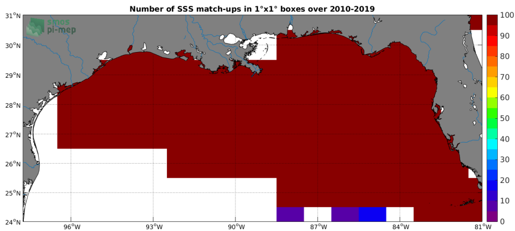
Figure 4: Number of SSS match-ups between TSG-SAMOS SSS and the SMOS-L3-CATDS-CPDC-V317-MONTHLY-25KM SSS product for the Mississippi river plume Pi-MEP region over 1^\circ \times 1^\circ boxes and for the full satellite product period.
