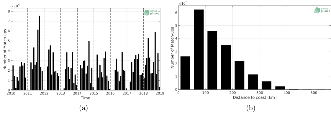
Figure 1: Number of match-ups between TSG-SAMOS and SMOS-L3-CATDS-CPDC-V317-MONTHLY-25KM SSS as a function of time (a) and as function of the distance to coast (b) over the Mississippi river plume Pi-MEP region and for the full satellite product period.
