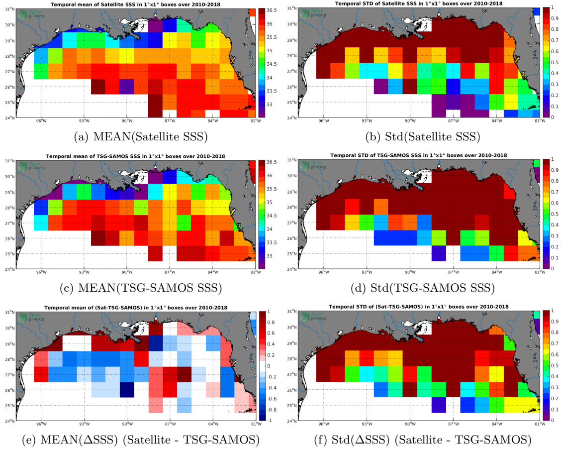
Figure 6: Temporal mean (left) and Std (right) of SSS from SMOS-L3-CATDS-CPDC-V317-MONTHLY-25KM (top), TSG-SAMOS (middle), and of \Delta SSS (Satellite - TSG-SAMOS). Only match-up pairs are used to generate these maps.
