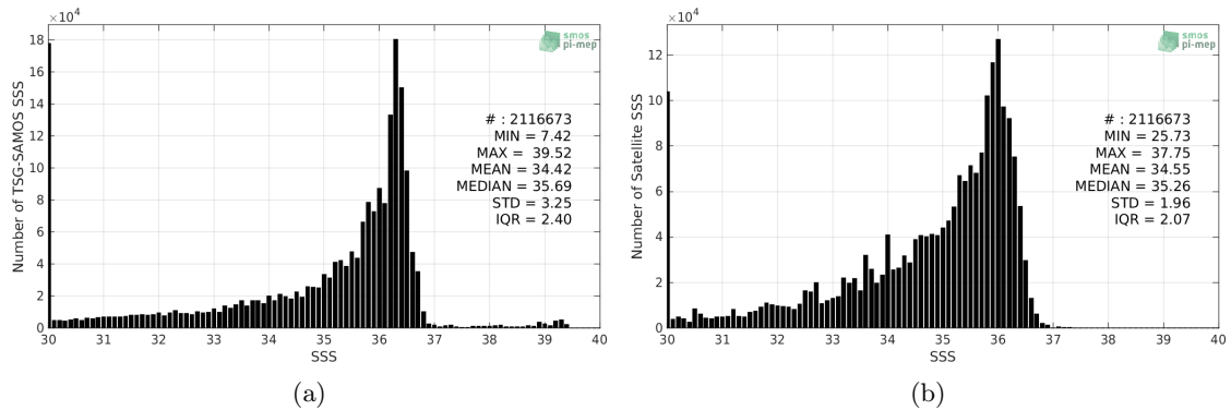
Figure 2: Histograms of SSS from TSG-SAMOS (a) and SMOS-L3-CATDS-CPDC-V317-MONTHLY-25KM (b) considering all match-up pairs per bins of 0.1 over the Mississippi river plume Pi-MEP region and for the full satellite product period.
