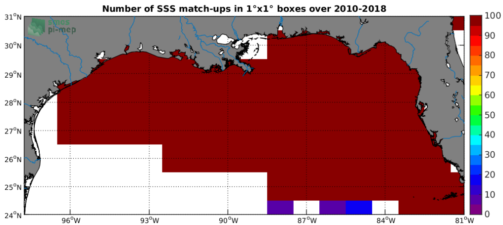
Figure 4: Number of SSS match-ups between TSG-SAMOS SSS and the SMOS-L3-CATDS-CPDC-V317-MONTHLY-25KM SSS product for the Mississippi river plume Pi-MEP region over 1^{\circ} \times 1^{\circ} boxes and for the full satellite product period.
