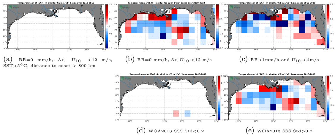
Figure 12: Temporal mean gridded over spatial boxes of size 1^\circ \times 1^\circ of \Delta SSS (SMOS-L3-CATDS-CPDC-V317-MONTHLY-25KM - TSG-SAMOS) for 5 different subdatasets corresponding to:RR=0 mm/h, 3 < U_{10} < 12 m/s, SST >5^\circ C, distance to coast > 800 km (a), RR=0 mm/h, 3 < U_{10} < 12 m/s (b), RR >1 mm/h and U_{10} < 4 m/s (c), WOA2013 SSS Std <0.2 (d), WOA2013 SSS Std >0.2 (e).
