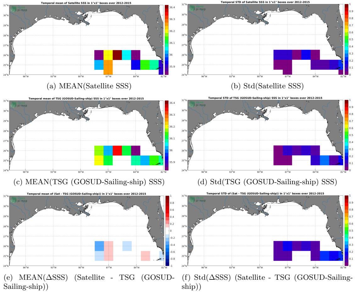
Figure 6: Temporal mean (left) and Std (right) of SSS from SMOS SSS L3 v317 - Monthly - 25 km (CATDS-CPDC) (top), TSG (GOSUD-Sailing-ship) (middle), and of \Delta SSS (Satellite - TSG (GOSUD-Sailing-ship)). Only match-up pairs are used to generate these maps.
