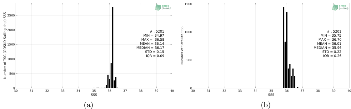
Figure 2: Histograms of SSS from TSG (GOSUD-Sailing-ship) (a) and SMOS SSS L3 v317 - Monthly - 25 km (CATDS-CPDC) (b) considering all match-up pairs per bins of 0.1 over the Mississippi river plume Pi-MEP region and for the full satellite product period.
