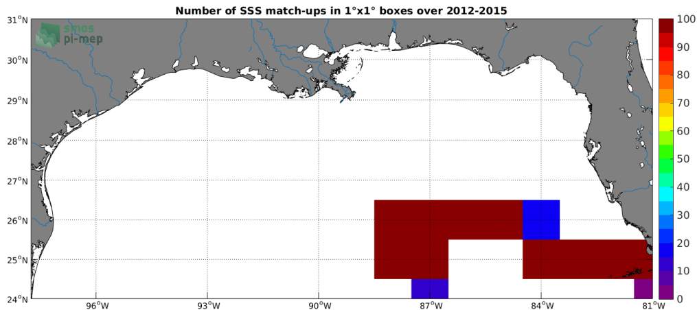
Figure 4: Number of SSS match-ups between TSG (GOSUD-Sailing-ship) SSS and the SMOS SSS L3 v317 - Monthly - 25 km (CATDS-CPDC) SSS product for the Mississippi river plume Pi-MEP region over 1^\circ \times 1^\circ boxes and for the full satellite product period.
