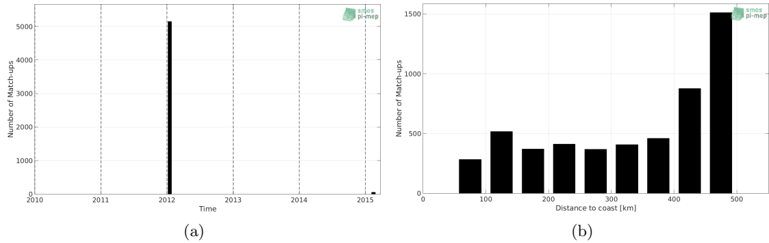
Figure 1: Number of match-ups between TSG (GOSUD-Sailing-ship) and SMOS SSS L3 v317 - Monthly - 25 km (CATDS-CPDC) SSS as a function of time (a) and as function of the distance to coast (b) over the Mississippi river plume Pi-MEP region and for the full satellite product period.
