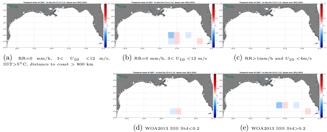
Figure 12: Temporal mean gridded over spatial boxes of size 1^\circ \times 1^\circ of \Delta SSS (SMOS SSS L3 v317 - Monthly - 25 km (CATDS-CPDC) - TSG (GOSUD-Sailing-ship)) for 5 different subdatasets corresponding to: RR=0 mm/h, 3 < U_{10} < 12 m/s, SST > 5^\circ\text{C} , distance to coast > 800 km (a), RR=0 mm/h, 3 < U_{10} < 12 m/s (b), RR > 1 mm/h and U_{10} < 4 m/s (c), WOA2013 SSS Std < 0.2 (d), WOA2013 SSS Std > 0.2 (e).
