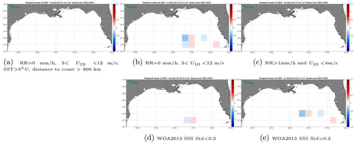
Figure 12: Temporal mean gridded over spatial boxes of size 1^{\circ}\times 1^{\circ} of \Delta SSS (SMOS SSS L3 v317 - Monthly - 25 km (CATDS-CPDC) - TSG (GOSUD-Sailing-ship)) for 5 different subdatasets corresponding to: RR=0 mm/h, 3 < U_{10} < 12 m/s, SST > 5^{\circ}\text{C} , distance to coast > 800 km (a), RR=0 mm/h, 3 < U_{10} < 12 m/s (b), RR > 1 mm/h and U_{10} < 4 m/s (c), WOA2013 SSS Std < 0.2 (d), WOA2013 SSS Std > 0.2 (e).
