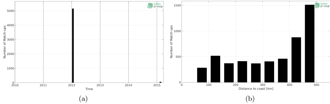
Figure 1: Number of match-ups between TSG-GOSUD-Sailing-ship and SMOS-L3-CATDS-CPDC-V317-MONTHLY-25KM SSS as a function of time (a) and as function of the distance to coast (b) over the Mississippi river plume Pi-MEP region and for the full satellite product period.
