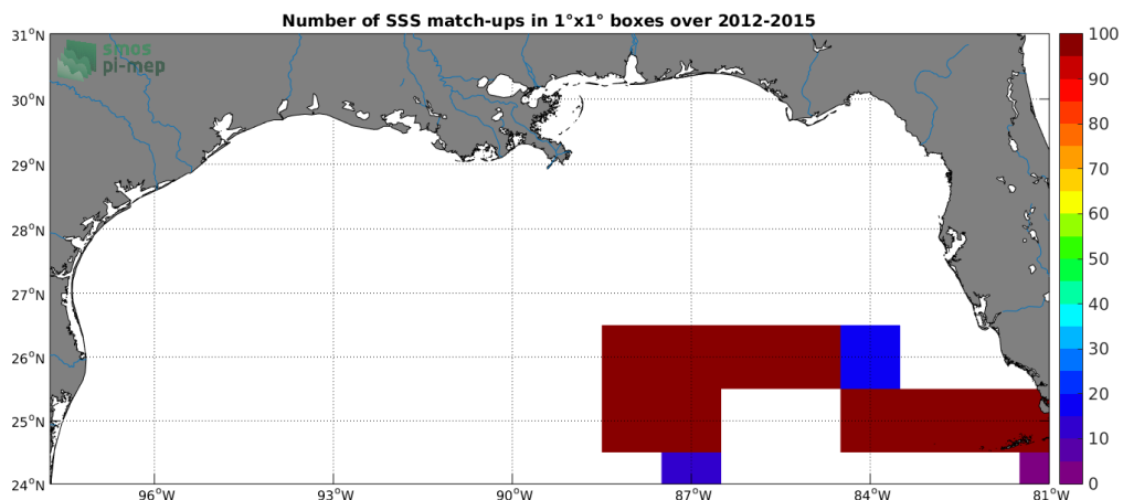
Figure 4: Number of SSS match-ups between TSG-GOSUD-Sailing-ship SSS and the SMOS-L3-CATDS-CPDC-V317-MONTHLY-25KM SSS product for the Mississippi river plume Pi-MEP region over 1^\circ \times 1^\circ boxes and for the full satellite product period.
