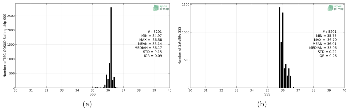
Figure 2: Histograms of SSS from TSG-GOSUD-Sailing-ship (a) and SMOS-L3-CATDS-CPDC-V317-MONTHLY-25KM (b) considering all match-up pairs per bins of 0.1 over the Mississippi river plume Pi-MEP region and for the full satellite product period.
