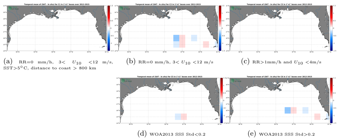
Figure 12: Temporal mean gridded over spatial boxes of size 1^\circ \times 1^\circ of \Delta SSS (SMOS-L3-CATDS-CPDC-V317-MONTHLY-25KM - TSG-GOSUD-Sailing-ship) for 5 different subdatasets corresponding to:RR=0 mm/h, 3 < U_{10} < 12 m/s, SST >5^\circ C, distance to coast > 800 km (a), RR=0 mm/h, 3 < U_{10} < 12 m/s (b), RR >1 mm/h and U_{10} < 4 m/s (c), WOA2013 SSS Std <0.2 (d), WOA2013 SSS Std >0.2 (e).
