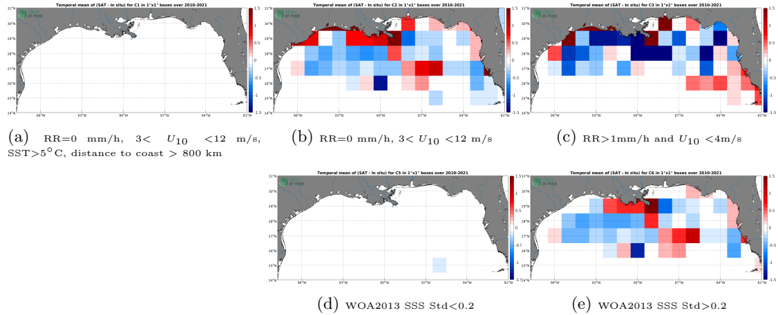
Figure 12: Temporal mean gridded over spatial boxes of size 1^{\circ}\times 1^{\circ} of \Delta\text{SSS} (SMOS SSS L3 v317 - 10 Days - 25 km (CATDS-CPDC) - TSG (SAMOS)) for 5 different subdatasets corresponding to:RR=0 mm/h, 3 < U_{10} < 12 m/s, SST >5^{\circ}\text{C} , distance to coast > 800 km (a), RR=0 mm/h, 3 < U_{10} < 12 m/s (b), RR >1 mm/h and U_{10} < 4 m/s (c), WOA2013 SSS Std <0.2 (d), WOA2013 SSS Std >0.2 (e).
