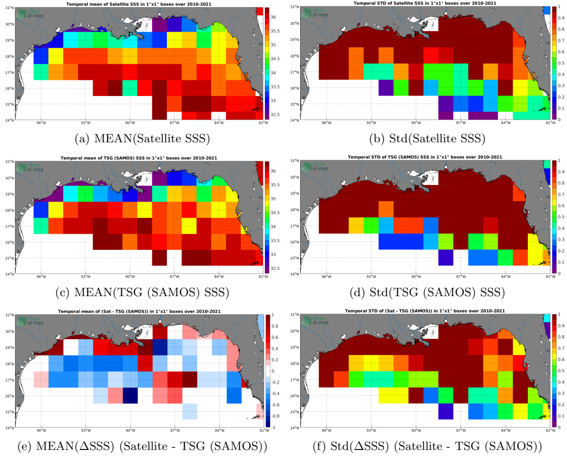
Figure 6: Temporal mean (left) and Std (right) of SSS from SMOS SSS L3 v317 - 10 Days - 25 km (CATDS-CPDC) (top), TSG (SAMOS) (middle), and of \Delta SSS (Satellite - TSG (SAMOS)). Only match-up pairs are used to generate these maps.
