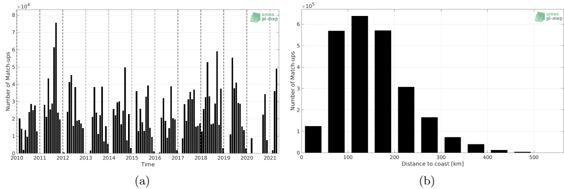
Figure 1: Number of match-ups between TSG (SAMOS) and SMOS SSS L3 v317 - 10 Days - 25 km (CATDS-CPDC) SSS as a function of time (a) and as function of the distance to coast (b) over the Mississippi river plume Pi-MEP region and for the full satellite product period.
