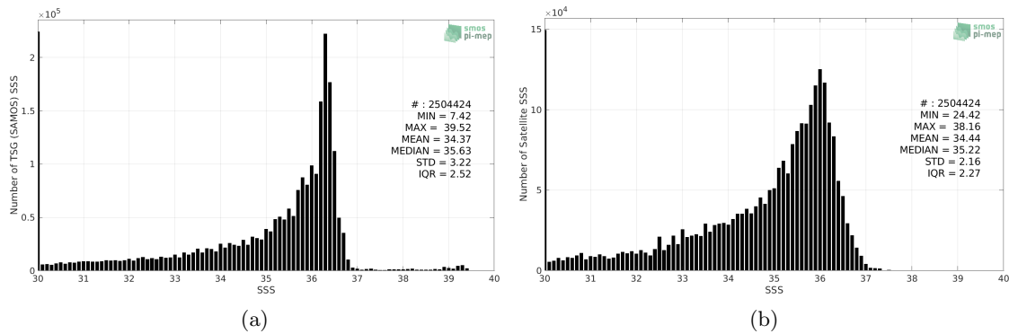
Figure 2: Histograms of SSS from TSG (SAMOS) (a) and SMOS SSS L3 v317 - 10 Days - 25 km (CATDS-CPDC) (b) considering all match-up pairs per bins of 0.1 over the Mississippi river plume Pi-MEP region and for the full satellite product period.
