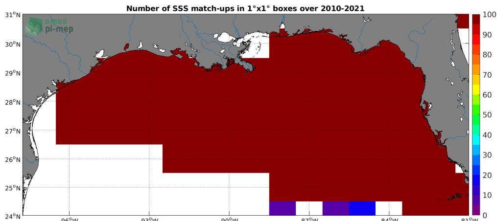
Figure 4: Number of SSS match-ups between TSG (SAMOS) SSS and the SMOS SSS L3 v317 - 10 Days - 25 km (CATDS-CPDC) SSS product for the Mississippi river plume Pi-MEP region over 1^\circ \times 1^\circ boxes and for the full satellite product period.
