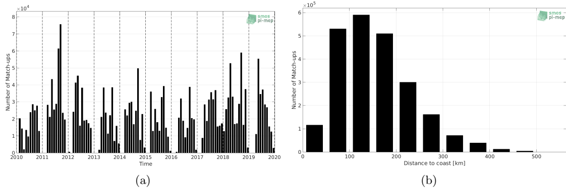
Figure 1: Number of match-ups between TSG-SAMOS and SMOS L3 v317 - 10 Days - 25 km (CATDS-CPDC) SSS as a function of time (a) and as function of the distance to coast (b) over the Mississippi river plume Pi-MEP region and for the full satellite product period.
