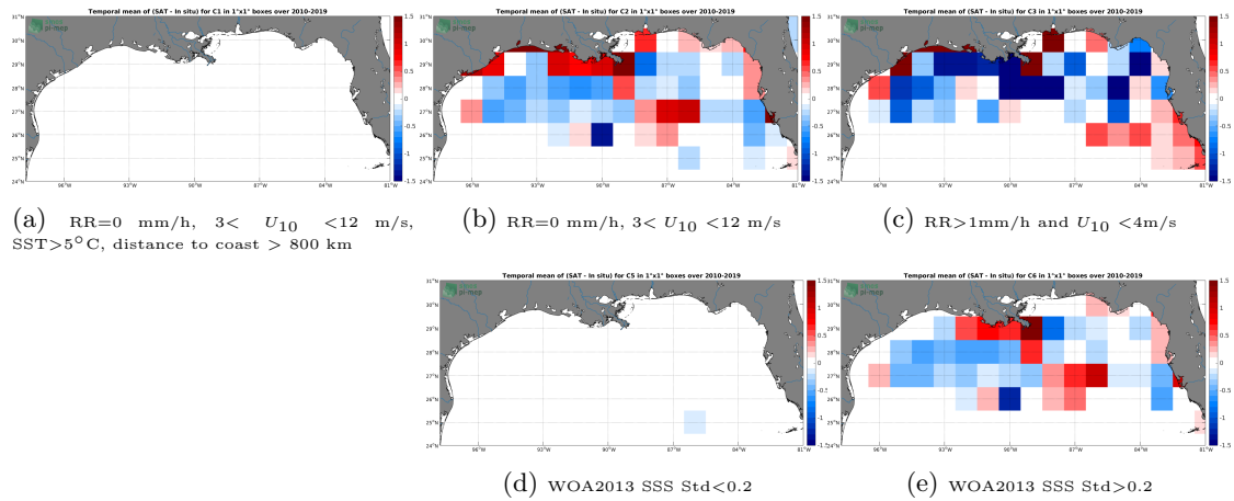
Figure 12: Temporal mean gridded over spatial boxes of size 1^{\circ}\times 1^{\circ} of \Delta\text{SSS} (SMOS L3 v317 - 10 Days - 25 km (CATDS-CPDC) - TSG-SAMOS) for 5 different subdatasets corresponding to:RR=0 mm/h, 3 < U_{10} < 12 m/s, SST >5^{\circ}\text{C} , distance to coast > 800 km (a), RR=0 mm/h, 3 < U_{10} < 12 m/s (b), RR >1 mm/h and U_{10} < 4 m/s (c), WOA2013 SSS Std <0.2 (d), WOA2013 SSS Std >0.2 (e).
