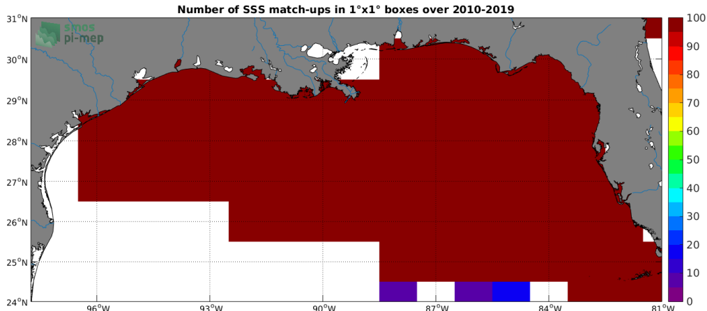
Figure 4: Number of SSS match-ups between TSG-SAMOS SSS and the SMOS L3 v317 - 10 Days - 25 km (CATDS-CPDC) SSS product for the Mississippi river plume Pi-MEP region over 1°x1° boxes and for the full satellite product period.
