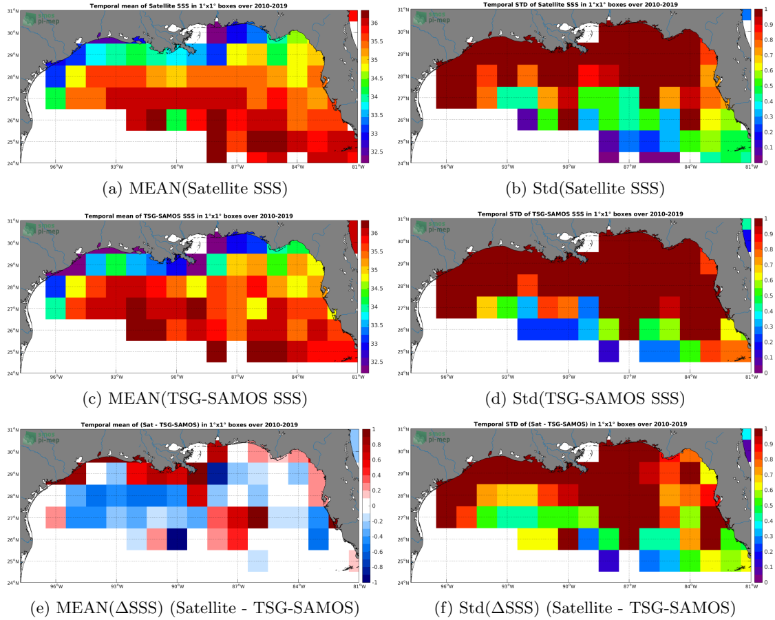
Figure 6: Temporal mean (left) and Std (right) of SSS from SMOS L3 v317 - 10 Days - 25 km (CATDS-CPDC) (top), TSG-SAMOS (middle), and of \Delta SSS (Satellite - TSG-SAMOS). Only match-up pairs are used to generate these maps.
