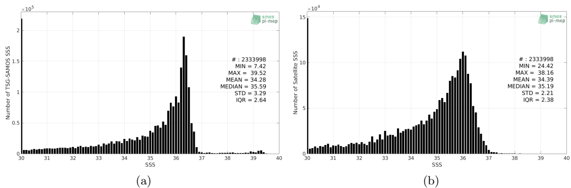
Figure 2: Histograms of SSS from TSG-SAMOS (a) and SMOS L3 v317 - 10 Days - 25 km (CATDS-CPDC) (b) considering all match-up pairs per bins of 0.1 over the Mississippi river plume Pi-MEP region and for the full satellite product period.
