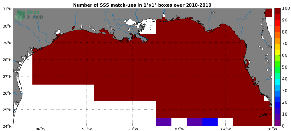
Figure 4: Number of SSS match-ups between TSG-SAMOS SSS and the SMOS-L3-CATDS-CPDC-V317-10DAYS-25KM SSS product for the Mississippi river plume Pi-MEP region over 1^\circ \times 1^\circ boxes and for the full satellite product period.
