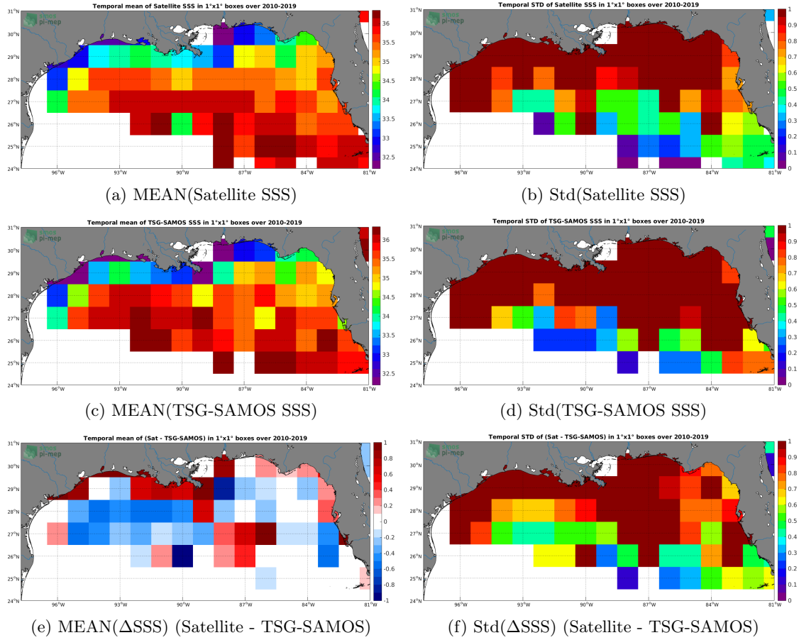
Figure 6: Temporal mean (left) and Std (right) of SSS from SMOS-L3-CATDS-CPDC-V317-10DAYS-25KM (top), TSG-SAMOS (middle), and of \Delta SSS (Satellite - TSG-SAMOS). Only match-up pairs are used to generate these maps.
