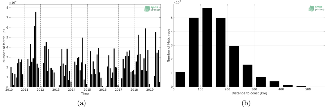
Figure 1: Number of match-ups between TSG-SAMOS and SMOS-L3-CATDS-CPDC-V317-10DAYS-25KM SSS as a function of time (a) and as function of the distance to coast (b) over the Mississippi river plume Pi-MEP region and for the full satellite product period.
