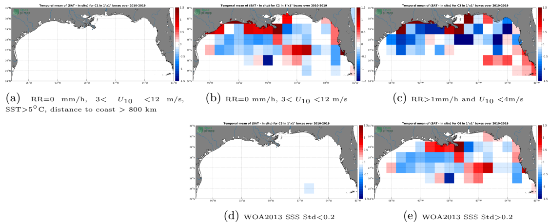
Figure 12: Temporal mean gridded over spatial boxes of size 1^\circ \times 1^\circ of \Delta SSS (SMOS-L3-CATDS-CPDC-V317-10DAYS-25KM - TSG-SAMOS) for 5 different subdatasets corresponding to:RR=0 mm/h, 3 < U_{10} < 12 m/s, SST > 5^\circ\text{C} , distance to coast > 800 km (a), RR=0 mm/h, 3 < U_{10} < 12 m/s (b), RR > 1 mm/h and U_{10} < 4 m/s (c), WOA2013 SSS Std < 0.2 (d), WOA2013 SSS Std > 0.2 (e).
