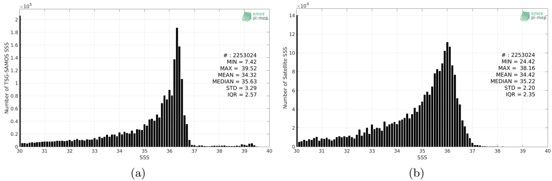
Figure 2: Histograms of SSS from TSG-SAMOS (a) and SMOS-L3-CATDS-CPDC-V317-10DAYS-25KM (b) considering all match-up pairs per bins of 0.1 over the Mississippi river plume Pi-MEP region and for the full satellite product period.
