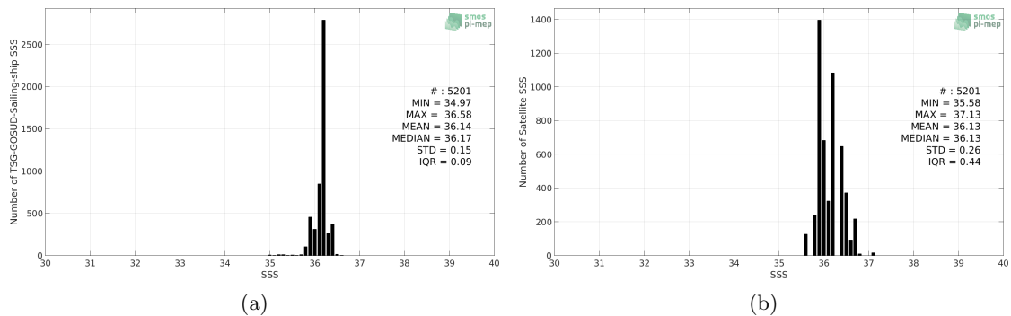
Figure 2: Histograms of SSS from TSG-GOSUD-Sailing-ship (a) and SMOS L3 v317 - 10 Days - 25 km (CATDS-CPDC) (b) considering all match-up pairs per bins of 0.1 over the Mississippi river plume Pi-MEP region and for the full satellite product period.
