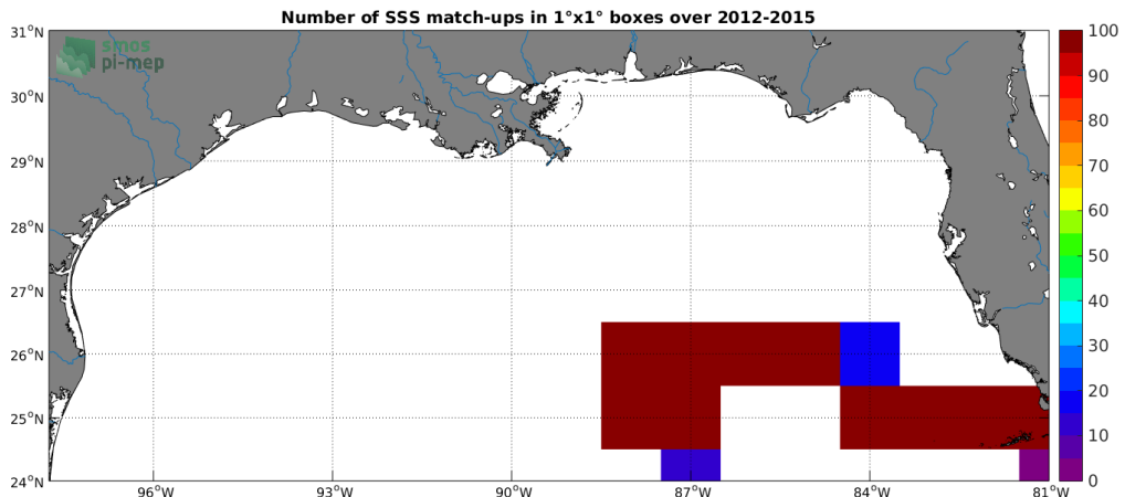
Figure 4: Number of SSS match-ups between TSG-GOSUD-Sailing-ship SSS and the SMOS L3 v317 - 10 Days - 25 km (CATDS-CPDC) SSS product for the Mississippi river plume Pi-MEP region over 1°x1° boxes and for the full satellite product period.
