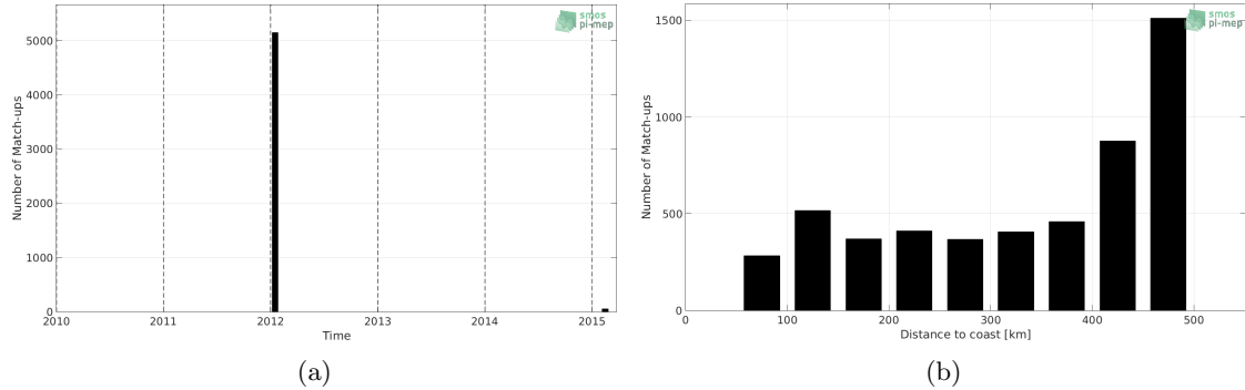
Figure 1: Number of match-ups between TSG-GOSUD-Sailing-ship and SMOS L3 v317 - 10 Days - 25 km (CATDS-CPDC) SSS as a function of time (a) and as function of the distance to coast (b) over the Mississippi river plume Pi-MEP region and for the full satellite product period.
