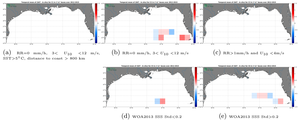
Figure 12: Temporal mean gridded over spatial boxes of size 1^{\circ}\times 1^{\circ} of \Delta SSS (SMOS L3 v317 - 10 Days - 25 km (CATDS-CPDC) - TSG-GOSUD-Sailing-ship) for 5 different subdatasets corresponding to:RR=0 mm/h, 3 < U_{10} < 12 m/s, SST >5^{\circ}\text{C} , distance to coast > 800 km (a), RR=0 mm/h, 3 < U_{10} < 12 m/s (b), RR >1 mm/h and U_{10} < 4 m/s (c), WOA2013 SSS Std <0.2 (d), WOA2013 SSS Std >0.2 (e).
