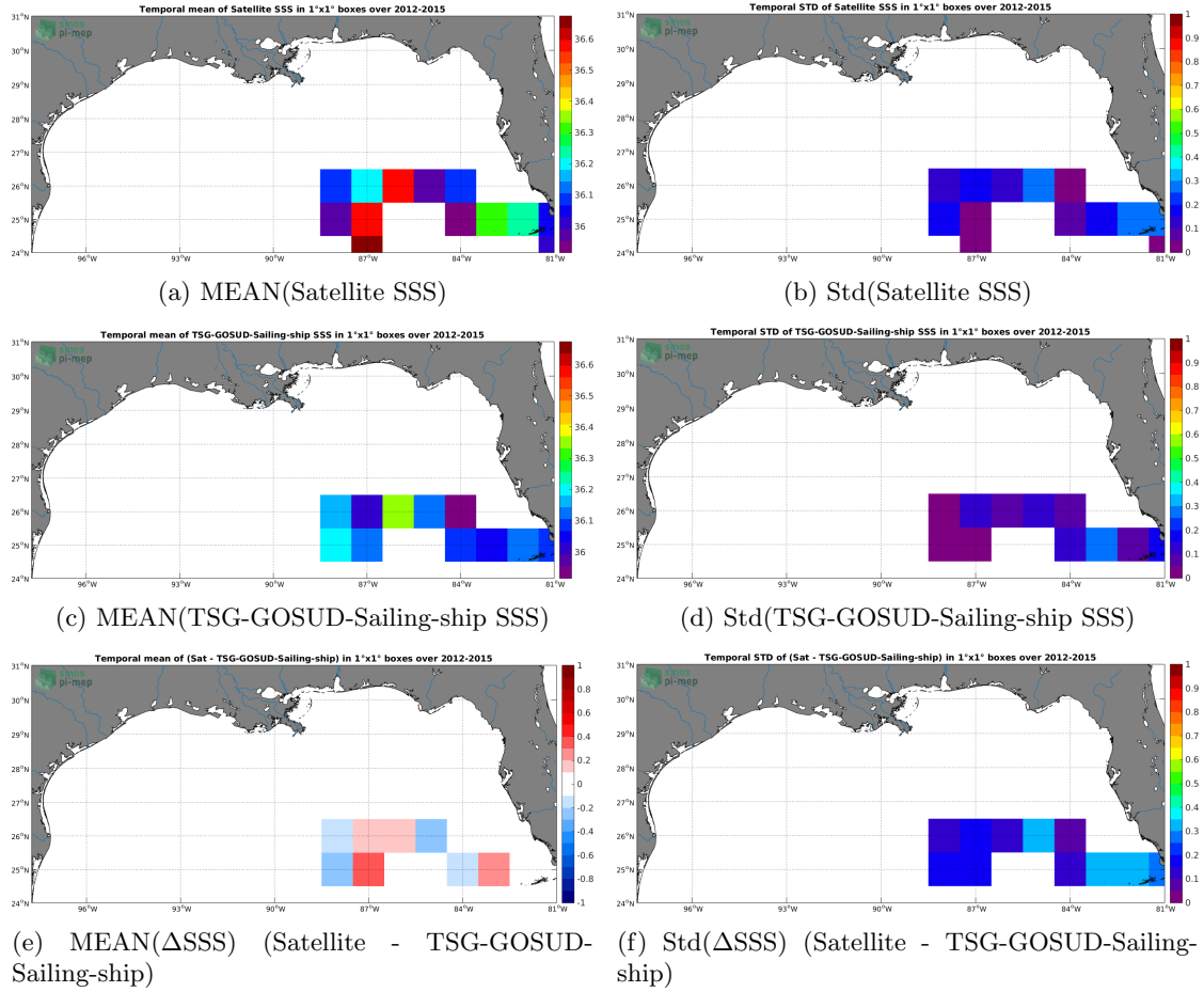
Figure 6: Temporal mean (left) and Std (right) of SSS from SMOS L3 v317 - 10 Days - 25 km (CATDS-CPDC) (top), TSG-GOSUD-Sailing-ship (middle), and of \Delta SSS (Satellite - TSG-GOSUD-Sailing-ship). Only match-up pairs are used to generate these maps.
