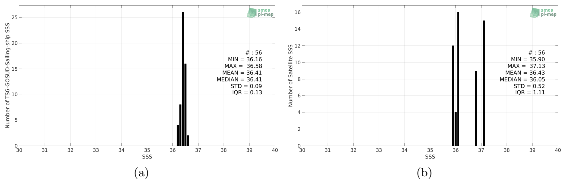
Figure 2: Histograms of SSS from TSG-GOSUD-Sailing-ship (a) and SMOS-L3-CATDS-CPDC-V317-10DAYS-25KM (b) considering all match-up pairs per bins of 0.1 over the Mississippi river plume Pi-MEP region and for the full satellite product period.
