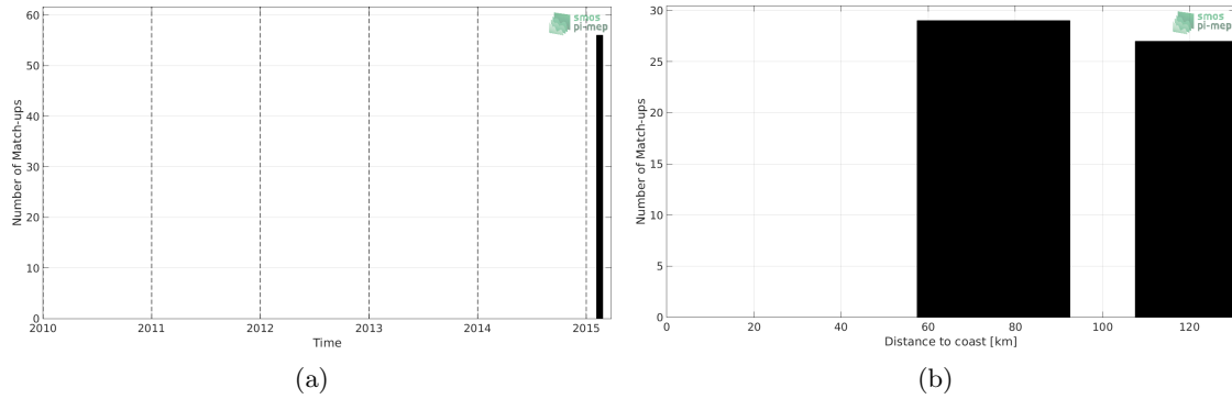
Figure 1: Number of match-ups between TSG-GOSUD-Sailing-ship and SMOS-L3-CATDS-CPDC-V317-10DAYS-25KM SSS as a function of time (a) and as function of the distance to coast (b) over the Mississippi river plume Pi-MEP region and for the full satellite product period.
