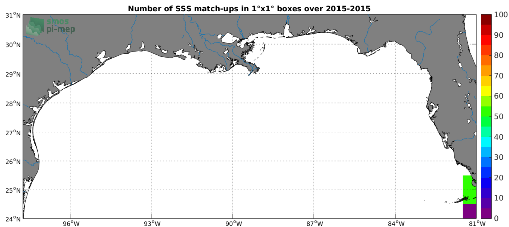
Figure 4: Number of SSS match-ups between TSG-GOSUD-Sailing-ship SSS and the SMOS-L3-CATDS-CPDC-V317-10DAYS-25KM SSS product for the Mississippi river plume Pi-MEP region over 1^\circ \times 1^\circ boxes and for the full satellite product period.
