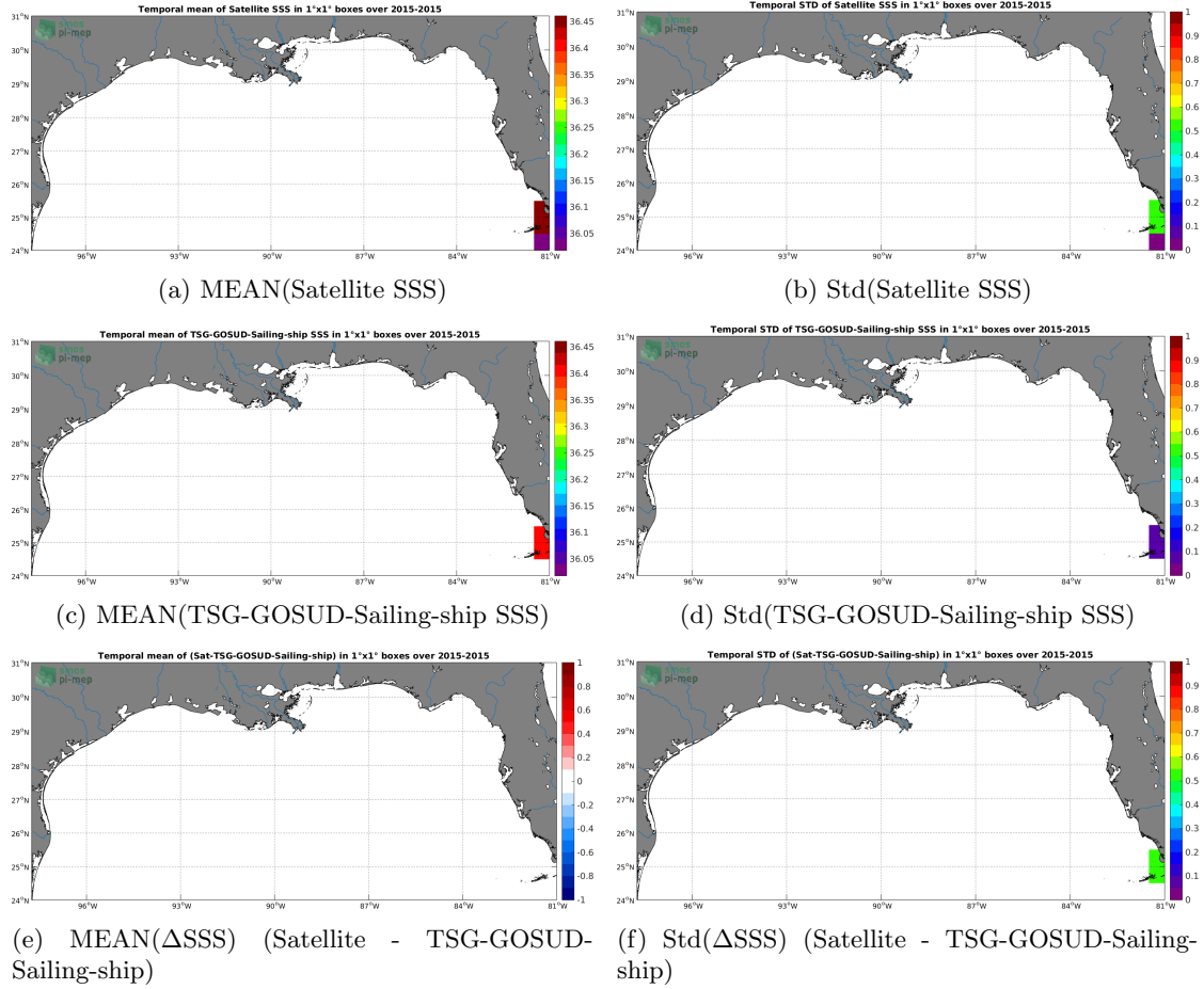
Figure 6: Temporal mean (left) and Std (right) of SSS from SMOS-L3-CATDS-CPDC-V317-10DAYS-25KM (top), TSG-GOSUD-Sailing-ship (middle), and of \Delta SSS (Satellite - TSG-GOSUD-Sailing-ship). Only match-up pairs are used to generate these maps.
