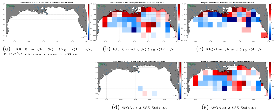
Figure 12: Temporal mean gridded over spatial boxes of size 1^\circ \times 1^\circ of \Delta SSS (SMOS-L3-CATDS-CPDC-V3-MONTHLY-25KM - TSG-SAMOS) for 5 different subdatasets corresponding to:RR=0 mm/h, 3 < U_{10} < 12 m/s, SST >5^\circ C, distance to coast > 800 km (a), RR=0 mm/h, 3 < U_{10} < 12 m/s (b), RR >1 mm/h and U_{10} < 4 m/s (c), WOA2013 SSS Std <0.2 (d), WOA2013 SSS Std >0.2 (e).
