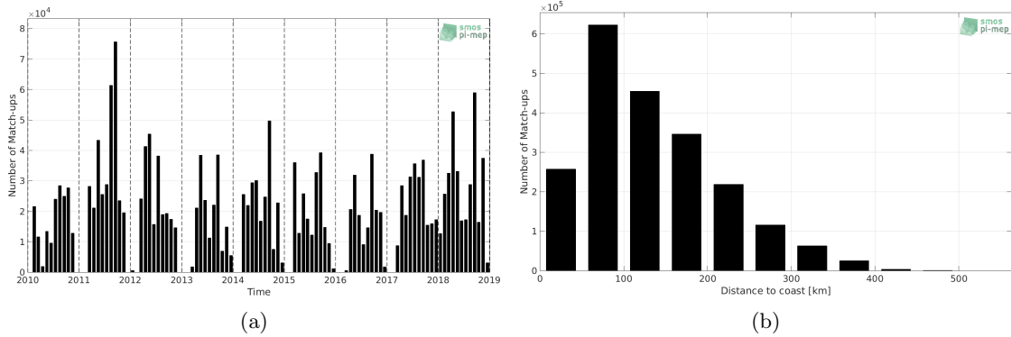
Figure 1: Number of match-ups between TSG-SAMOS and SMOS-L3-CATDS-CPDC-V3-10DAYS-25KM SSS as a function of time (a) and as function of the distance to coast (b) over the Mississippi river plume Pi-MEP region and for the full satellite product period.
