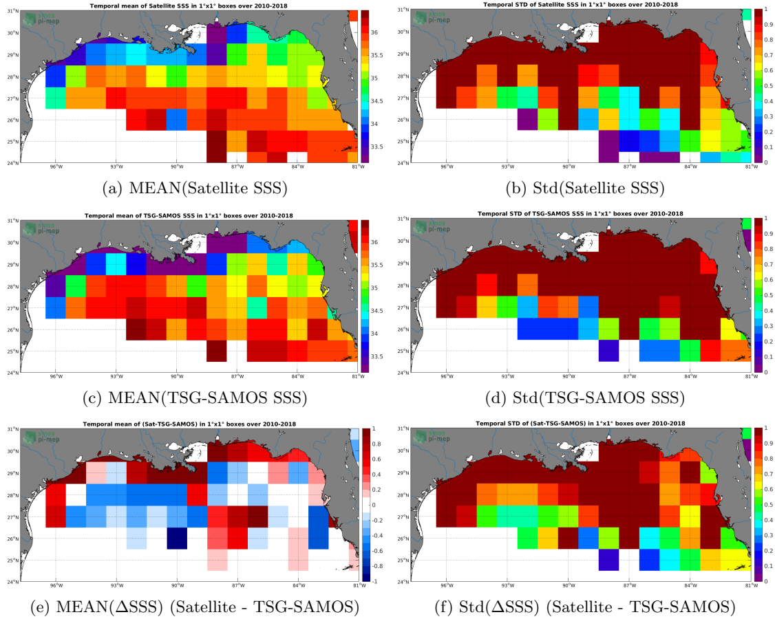
Figure 6: Temporal mean (left) and Std (right) of SSS from SMOS-L3-CATDS-CPDC-V3-10DAYS-25KM (top), TSG-SAMOS (middle), and of \Delta SSS (Satellite - TSG-SAMOS). Only match-up pairs are used to generate these maps.
