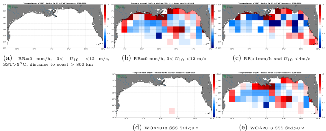
Figure 12: Temporal mean gridded over spatial boxes of size 1^\circ \times 1^\circ of \Delta SSS (SMOS-L3-CATDS-CPDC-V3-10DAYS-25KM - TSG-SAMOS) for 5 different subdatasets corresponding to:RR=0 mm/h, 3 < U_{10} < 12 m/s, SST > 5^\circ C , distance to coast > 800 km (a), RR=0 mm/h, 3 < U_{10} < 12 m/s (b), RR > 1 mm/h and U_{10} < 4 m/s (c), WOA2013 SSS Std < 0.2 (d), WOA2013 SSS Std > 0.2 (e).
