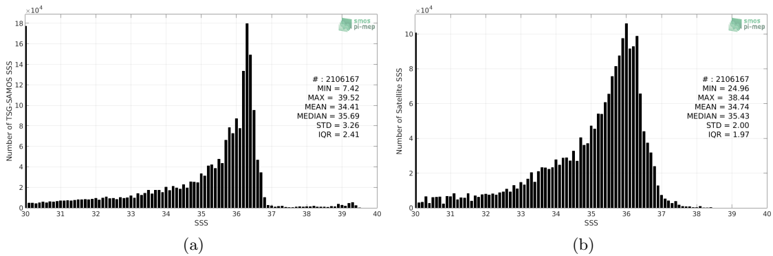
Figure 2: Histograms of SSS from TSG-SAMOS (a) and SMOS-L3-CATDS-CPDC-V3-10DAYS-25KM (b) considering all match-up pairs per bins of 0.1 over the Mississippi river plume Pi-MEP region and for the full satellite product period.
