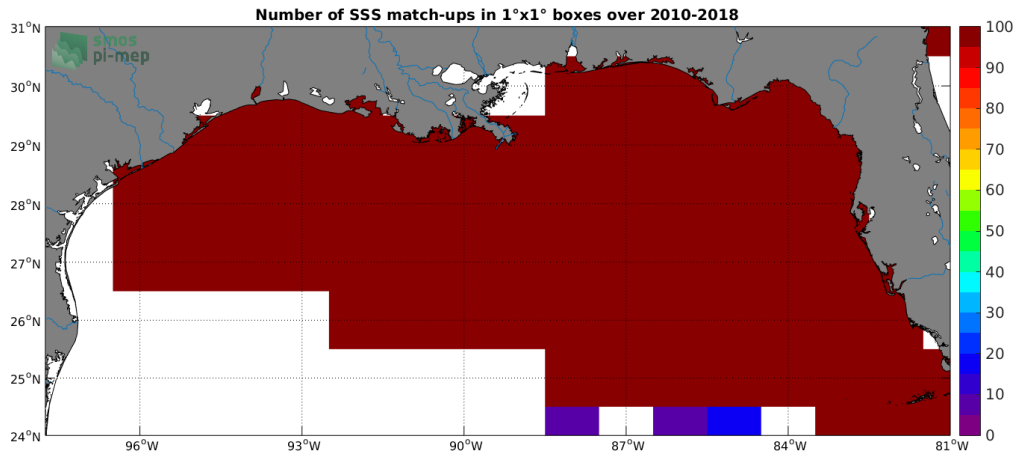
Figure 4: Number of SSS match-ups between TSG-SAMOS SSS and the SMOS-L3-CATDS-CPDC-V3-10DAYS-25KM SSS product for the Mississippi river plume Pi-MEP region over 1^\circ \times 1^\circ boxes and for the full satellite product period.
