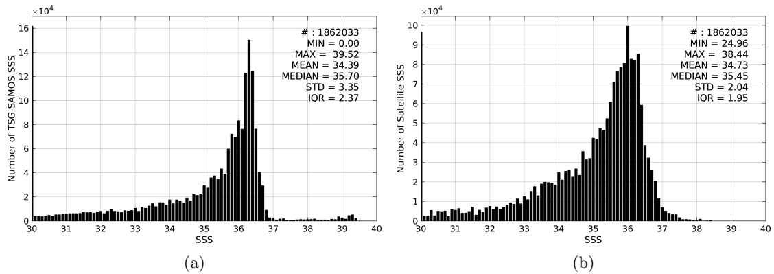
Figure 2: Histograms of SSS from TSG-SAMOS (a) and SMOS-L3-CATDS-CPDC-V3-10DAYS-25KM (b) considering all match-up pairs per bins of 0.1 over the Mississippi river plume Pi-MEP region and for the full satellite product period.
