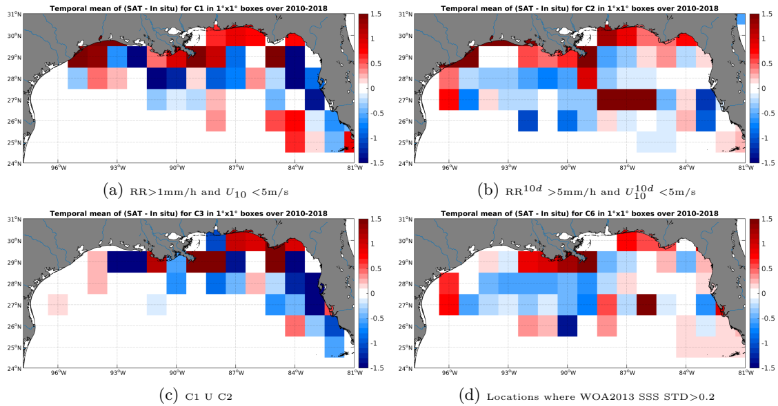
Figure 12: Temporal mean gridded over spatial boxes of size 1^\circ \times 1^\circ of \Delta SSS (SMOS-L3-CATDS-CPDC-V3-10DAYS-25KM - TSG-SAMOS) for 4 different subdatasets corresponding to:RR > 1 mm/h and U_{10} < 5 m/s (a), RR^{10d} > 5 mm/h and U_{10}^{10d} < 5 m/s (b), C1 U C2 (c),Locations where WOA2013 SSS STD > 0.2 (d).
