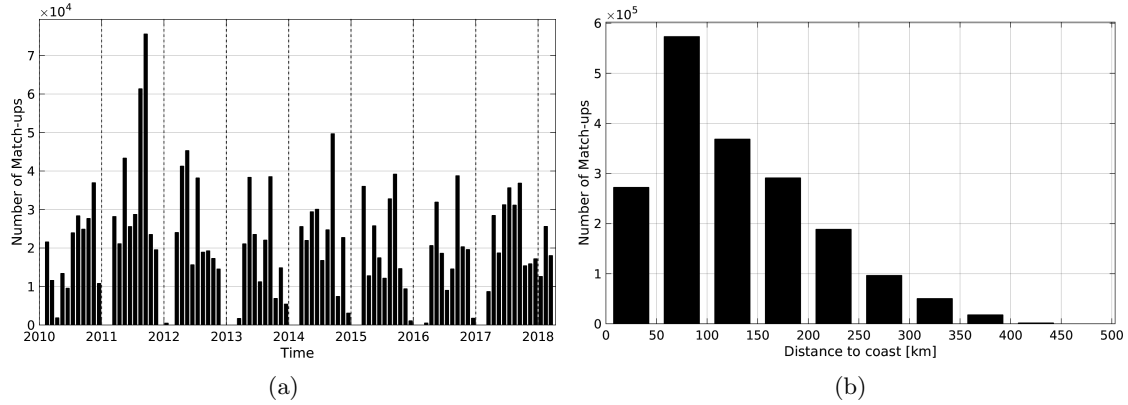
Figure 1: Number of match-ups between TSG-SAMOS and SMOS-L3-CATDS-CPDC-V3-10DAYS-25KM SSS as a function of time (a) and as function of the distance to coast (b) over the Mississippi river plume Pi-MEP region and for the full satellite product period.
