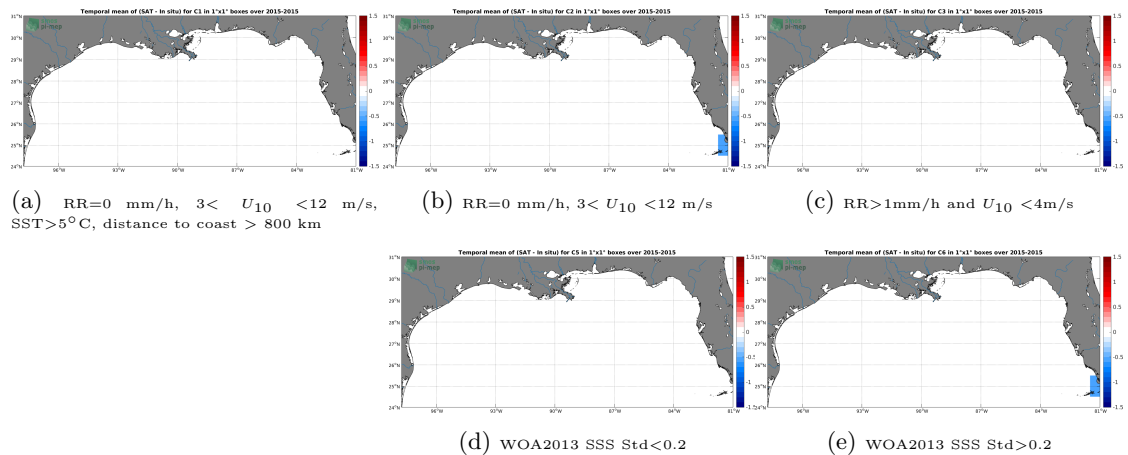
Figure 12: Temporal mean gridded over spatial boxes of size 1^\circ \times 1^\circ of \Delta SSS (SMOS-L3-CATDS-CPDC-V3-10DAYS-25KM - TSG-GOSUD-Sailing-ship) for 5 different subdatasets corresponding to:RR=0 mm/h, 3 < U_{10} < 12 m/s, SST >5^\circ C, distance to coast > 800 km (a), RR=0 mm/h, 3 < U_{10} < 12 m/s (b), RR >1 mm/h and U_{10} < 4 m/s (c), WOA2013 SSS Std <0.2 (d), WOA2013 SSS Std >0.2 (e).
