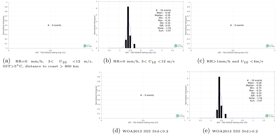
Figure 13: Normalized histogram of \Delta\text{SSS} (SMOS-L3-CATDS-CPDC-V3-10DAYS-25KM - TSG-GOSUD-Sailing-ship) for 5 different subdatasets corresponding to: RR=0 mm/h, 3 < U_{10} < 12 m/s, SST > 5^\circ\text{C} , distance to coast > 800 km (a), RR=0 mm/h, 3 < U_{10} < 12 m/s (b), RR > 1\text{mm/h} and U_{10} < 4\text{m/s} (c), WOA2013 SSS Std < 0.2 (d), WOA2013 SSS Std > 0.2 (e).
