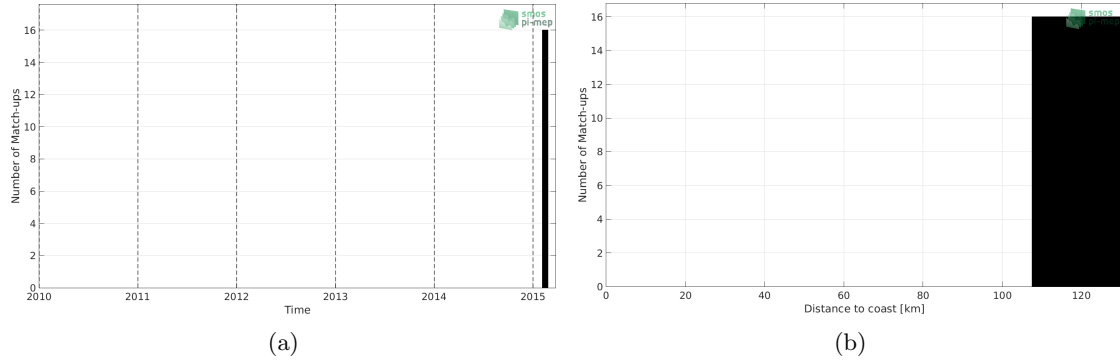
Figure 1: Number of match-ups between TSG-GOSUD-Sailing-ship and SMOS-L3-CATDS-CPDC-V3-10DAYS-25KM SSS as a function of time (a) and as function of the distance to coast (b) over the Mississippi river plume Pi-MEP region and for the full satellite product period.
