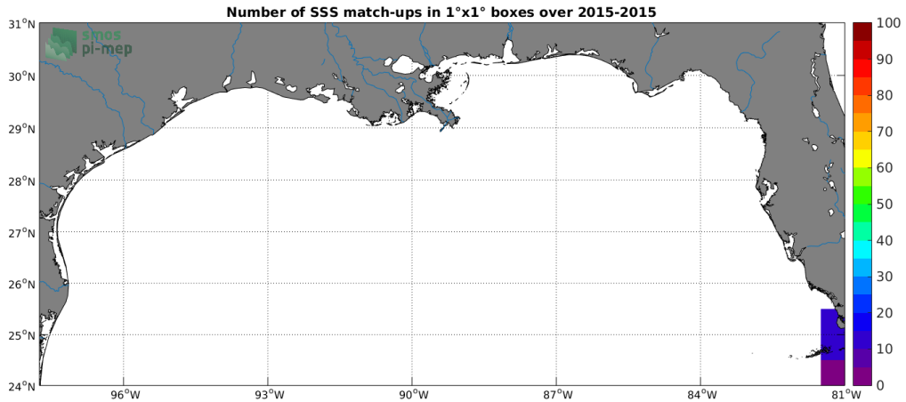
Figure 4: Number of SSS match-ups between TSG-GOSUD-Sailing-ship SSS and the SMOS-L3-CATDS-CPDC-V3-10DAYS-25KM SSS product for the Mississippi river plume Pi-MEP region over 1^{\circ} \times 1^{\circ} boxes and for the full satellite product period.
