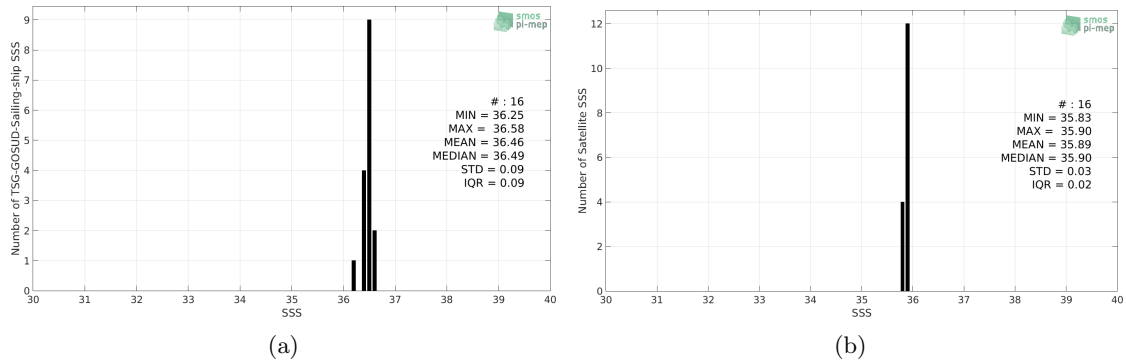
Figure 2: Histograms of SSS from TSG-GOSUD-Sailing-ship (a) and SMOS-L3-CATDS-CPDC-V3-10DAYS-25KM (b) considering all match-up pairs per bins of 0.1 over the Mississippi river plume Pi-MEP region and for the full satellite product period.
