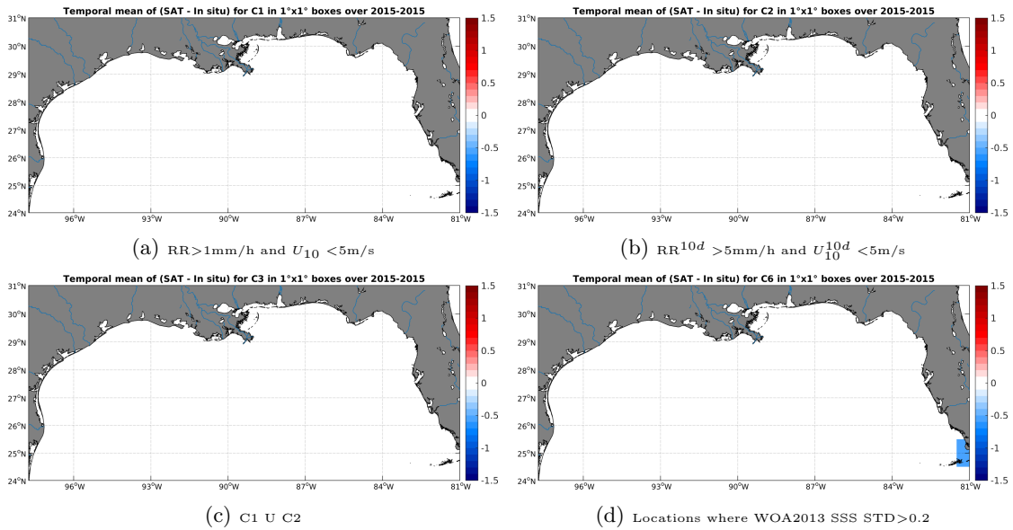
Figure 12: Temporal mean gridded over spatial boxes of size 1^\circ \times 1^\circ of \Delta SSS (SMOS-L3-CATDS-CPDC-V3-10DAYS-25KM - TSG-GOSUD-Sailing-ship) for 4 different subdatasets corresponding to: RR > 1\text{mm/h} and U_{10} < 5\text{m/s} (a), RR^{10d} > 5\text{mm/h} and U_{10}^{10d} < 5\text{m/s} (b), C1 U C2 (c), Locations where WOA2013 SSS STD > 0.2 (d).
