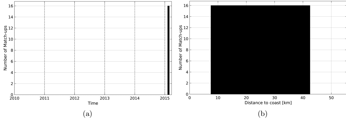
Figure 1: Number of match-ups between TSG-GOSUD-Sailing-ship and SMOS-L3-CATDS-CPDC-V3-10DAYS-25KM SSS as a function of time (a) and as function of the distance to coast (b) over the Mississippi river plume Pi-MEP region and for the full satellite product period.
