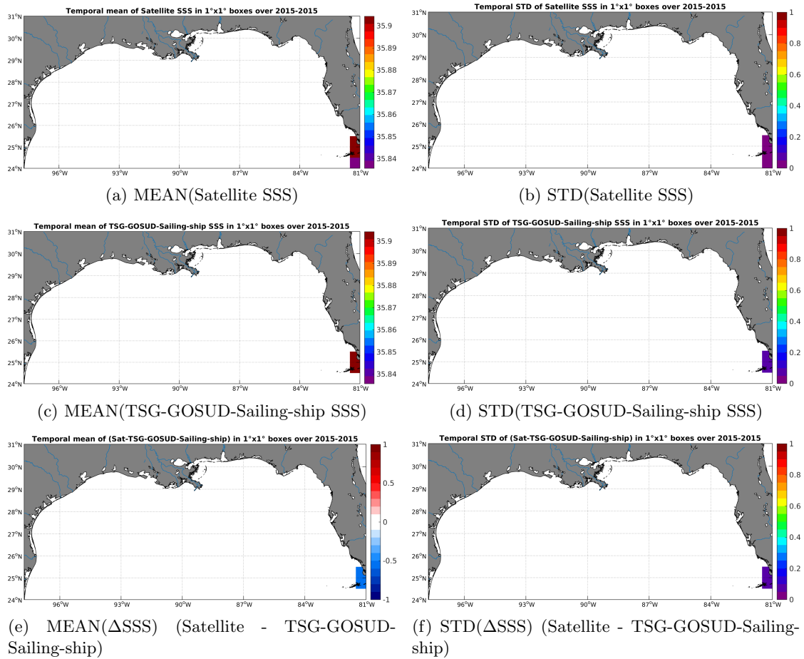
Figure 6: Temporal mean (left) and STD (right) of SSS from SMOS-L3-CATDS-CPDC-V3-10DAYS-25KM (top), TSG-GOSUD-Sailing-ship (middle), and of \Delta SSS (Satellite - TSG-GOSUD-Sailing-ship). Only match-up pairs are used to generate these maps.
