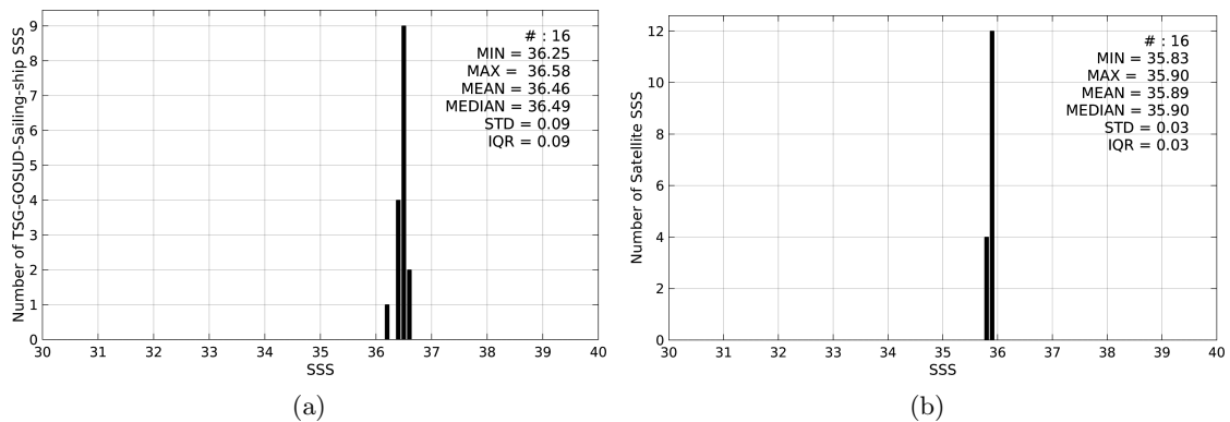
Figure 2: Histograms of SSS from TSG-GOSUD-Sailing-ship (a) and SMOS-L3-CATDS-CPDC-V3-10DAYS-25KM (b) considering all match-up pairs per bins of 0.1 over the Mississippi river plume Pi-MEP region and for the full satellite product period.
