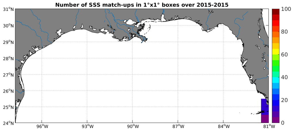
Figure 4: Number of SSS match-ups between TSG-GOSUD-Sailing-ship SSS and the SMOS-L3-CATDS-CPDC-V3-10DAYS-25KM SSS product for the Mississippi river plume Pi-MEP region over 1^\circ \times 1^\circ boxes and for the full satellite product period.
