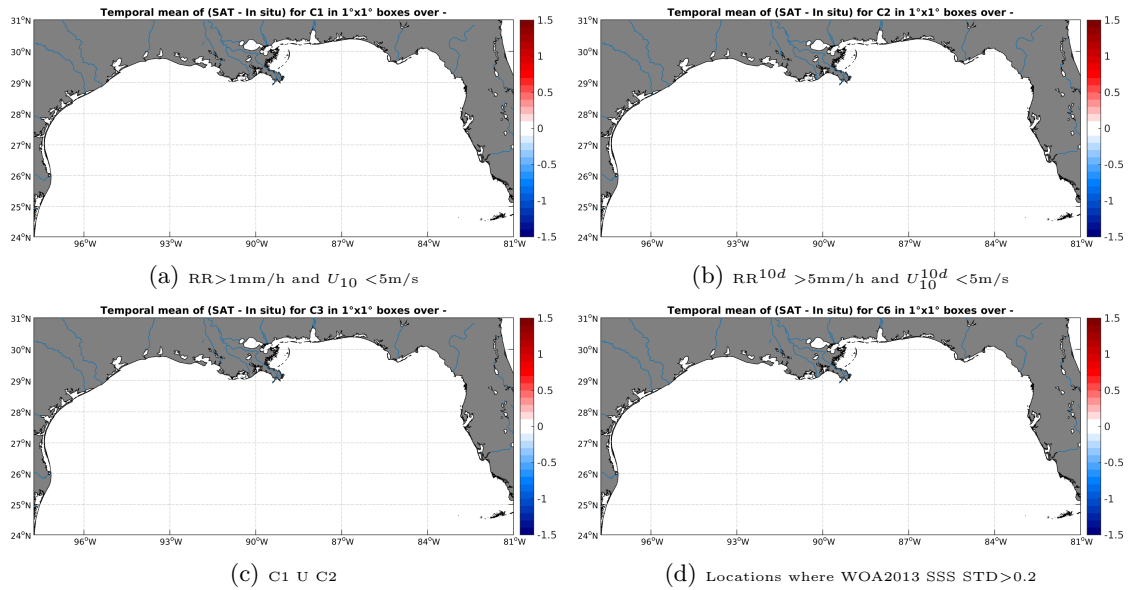
Figure 12: Temporal mean gridded over spatial boxes of size 1^\circ \times 1^\circ of \Delta SSS (SMOS-L3-CATDS-CPDC-V3-10DAYS-25KM - TSG-GOSUD-Research-vessel) for 4 different subdatasets corresponding to:RR > 1 mm/h and U_{10} < 5 m/s (a), RR 10d > 5 mm/h and U_{10}^{10d} < 5 m/s (b), C1 U C2 (c),Locations where WOA2013 SSS STD > 0.2 (d).
