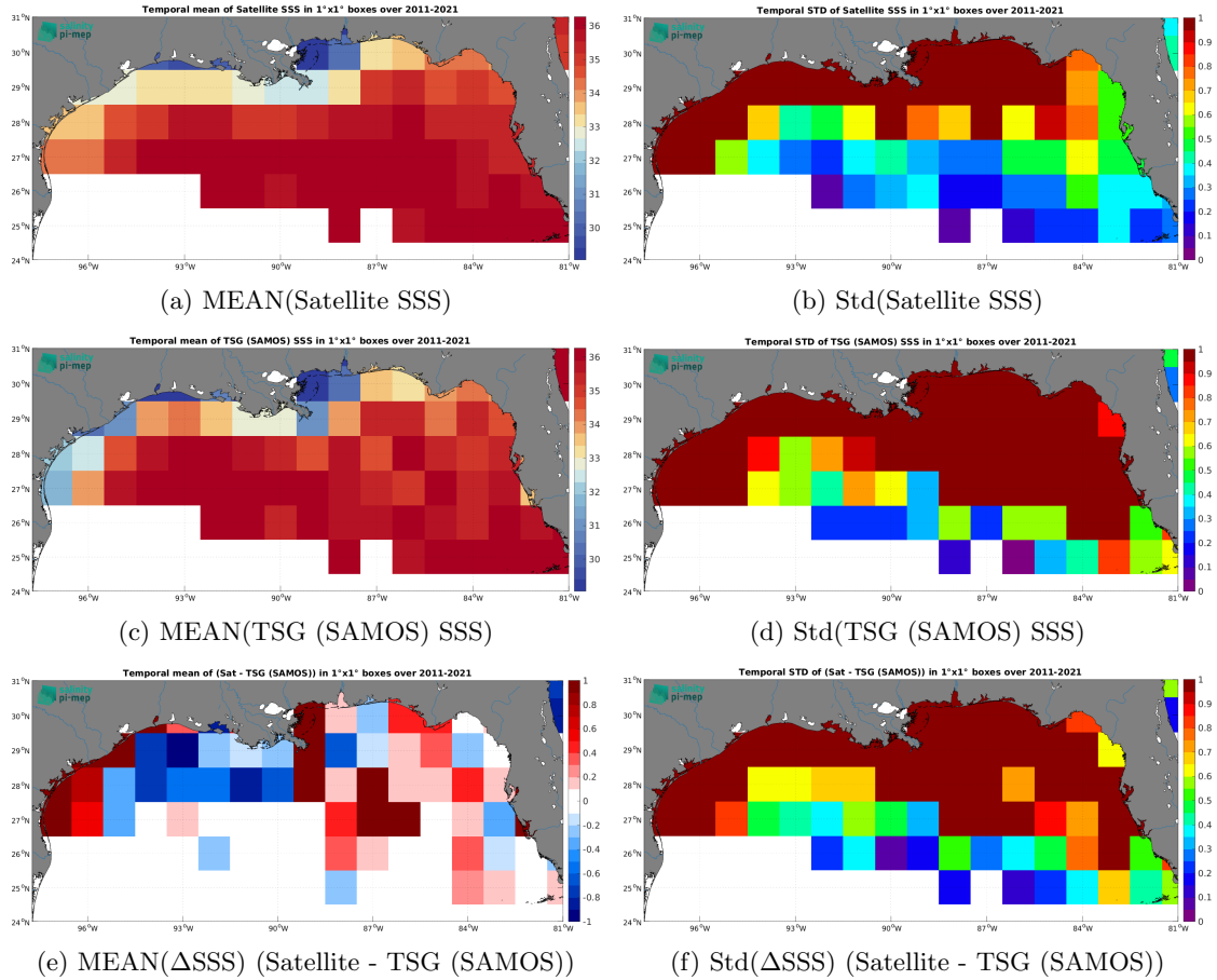
Figure 6: Temporal mean (left) and Std (right) of SSS from SMOS SSS L3 v2 - 9-Days (BEC) (top), TSG (SAMOS) (middle), and of \Delta\text{SSS} (Satellite - TSG (SAMOS)). Only match-up pairs are used to generate these maps.
