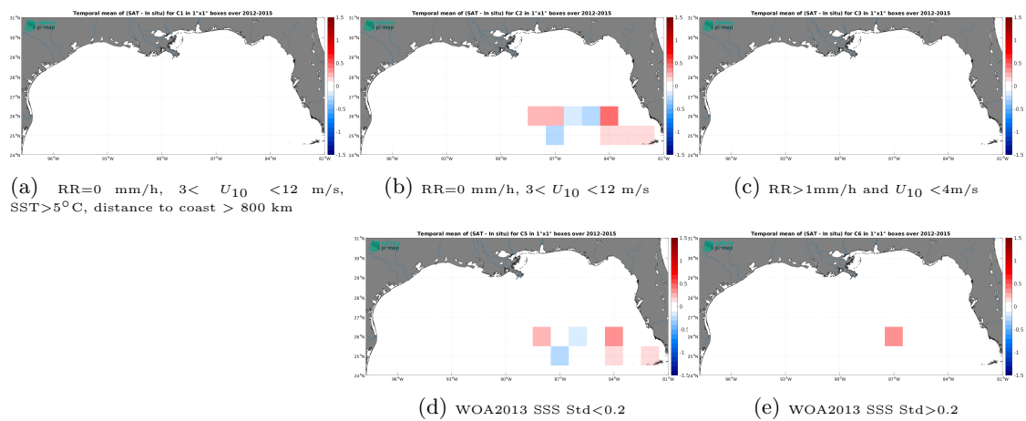
Figure 14: Temporal mean gridded over spatial boxes of size 1^\circ \times 1^\circ of \Delta SSS (SMOS SSS L3 v2 - 9-Days (BEC) - TSG (GOSUD-Sailing-ship)) for 5 different subdatasets corresponding to: RR=0 mm/h, 3 < U_{10} < 12 m/s, SST > 5^\circ\text{C} , distance to coast > 800 km (a), RR=0 mm/h, 3 < U_{10} < 12 m/s (b), RR > 1 mm/h and U_{10} < 4 m/s (c), WOA2013 SSS Std < 0.2 (d), WOA2013 SSS Std > 0.2 (e).
