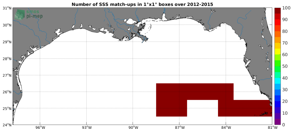
Figure 4: Number of SSS match-ups between TSG (GOSUD-Sailing-ship) SSS and the SMOS SSS L3 v2 - 9-Days (BEC) SSS product for the Mississippi river plume Pi-MEP region over 1°x1° boxes and for the full satellite product period.
