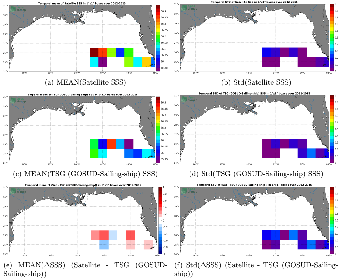
Figure 6: Temporal mean (left) and Std (right) of SSS from SMOS SSS L3 v2 - 9-Days (BEC) (top), TSG (GOSUD-Sailing-ship) (middle), and of \Delta SSS (Satellite - TSG (GOSUD-Sailing-ship)). Only match-up pairs are used to generate these maps.
