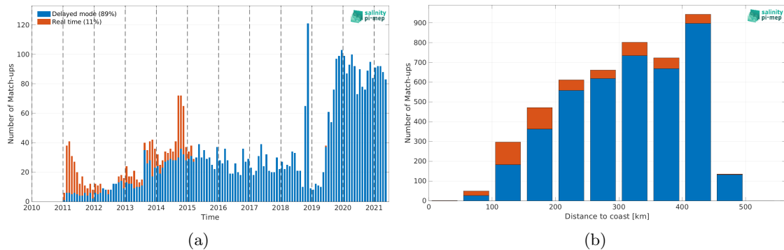
Figure 2: Number of match-ups between Argo and SMOS SSS L3 v2 - 9-Days (BEC) SSS as a function of time (a) and as function of the distance to coast (b) over the Mississippi river plume Pi-MEP region and for the full satellite product period.
