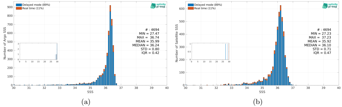
Figure 3: Histograms of SSS from Argo (a) and SMOS SSS L3 v2 - 9-Days (BEC) (b) considering all match-up pairs per bins of 0.1 over the Mississippi river plume Pi-MEP region and for the full satellite product period.
