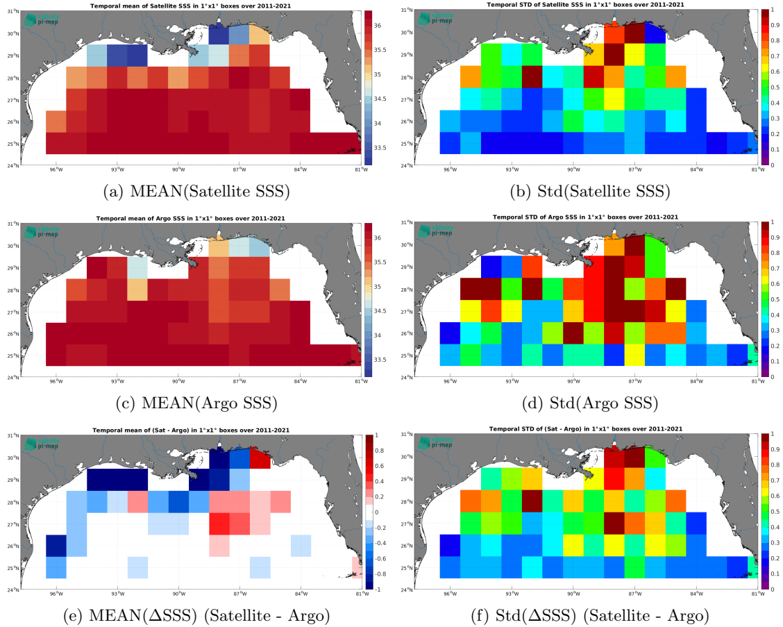
Figure 7: Temporal mean (left) and Std (right) of SSS from SMOS SSS L3 v2 - 9-Days (BEC) (top), Argo (middle), and of \Delta\text{SSS} (Satellite - Argo). Only match-up pairs are used to generate these maps.
