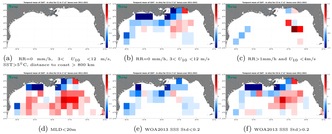
Figure 14: Temporal mean gridded over spatial boxes of size 1^\circ \times 1^\circ of \Delta SSS (SMOS SSS L3 v2 - 9-Days (BEC) - Argo) for 6 different subdatasets corresponding to:RR=0 mm/h, 3 < U_{10} < 12 m/s, SST>5°C, distance to coast > 800 km (a), RR=0 mm/h, 3 < U_{10} < 12 m/s (b), RR>1mm/h and U_{10} < 4 m/s (c),MLD<20m (d),WOA2013 SSS Std<0.2 (e),WOA2013 SSS Std>0.2 (f).
