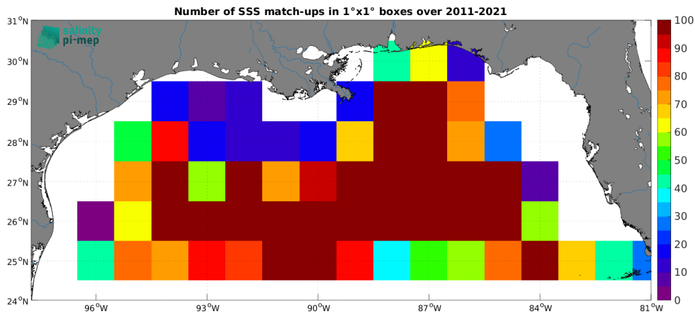
Figure 5: Number of SSS match-ups between Argo SSS and the SMOS SSS L3 v2 - 9-Days (BEC) SSS product for the Mississippi river plume Pi-MEP region over 1^\circ \times 1^\circ boxes and for the full satellite product period.
