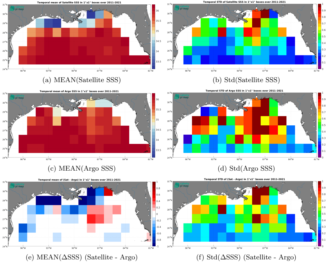
Figure 6: Temporal mean (left) and Std (right) of SSS from SMOS SSS L3 v2 - 9-Days (BEC) (top), Argo (middle), and of \Delta\text{SSS} (Satellite - Argo). Only match-up pairs are used to generate these maps.
