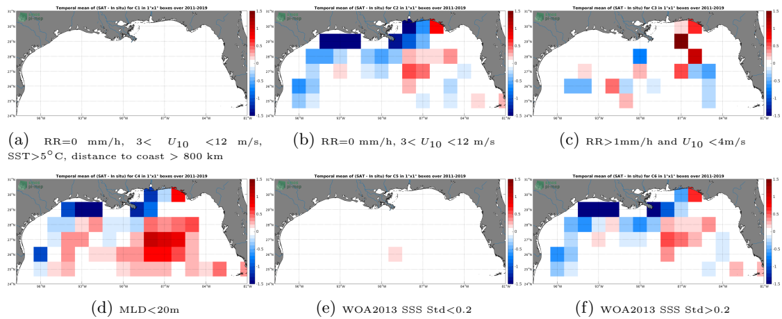
Figure 12: Temporal mean gridded over spatial boxes of size 1^{\circ}\times 1^{\circ} of \Delta\text{SSS} (SMOS L3 v2 - 9-Days (BEC) - Argo) for 6 different subdatasets corresponding to:RR=0 mm/h, 3 < U_{10} < 12 m/s, SST > 5^{\circ}\text{C} , distance to coast > 800 km (a), RR=0 mm/h, 3 < U_{10} < 12 m/s (b), RR > 1\text{mm/h} and U_{10} < 4\text{m/s} (c),MLD < 20\text{m} (d),WOA2013 SSS Std < 0.2 (e),WOA2013 SSS Std > 0.2 (f).
