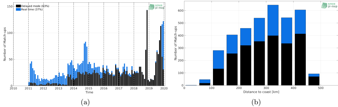
Figure 1: Number of match-ups between Argo and SMOS L3 v2 - 9-Days (BEC) SSS as a function of time (a) and as function of the distance to coast (b) over the Mississippi river plume Pi-MEP region and for the full satellite product period.
