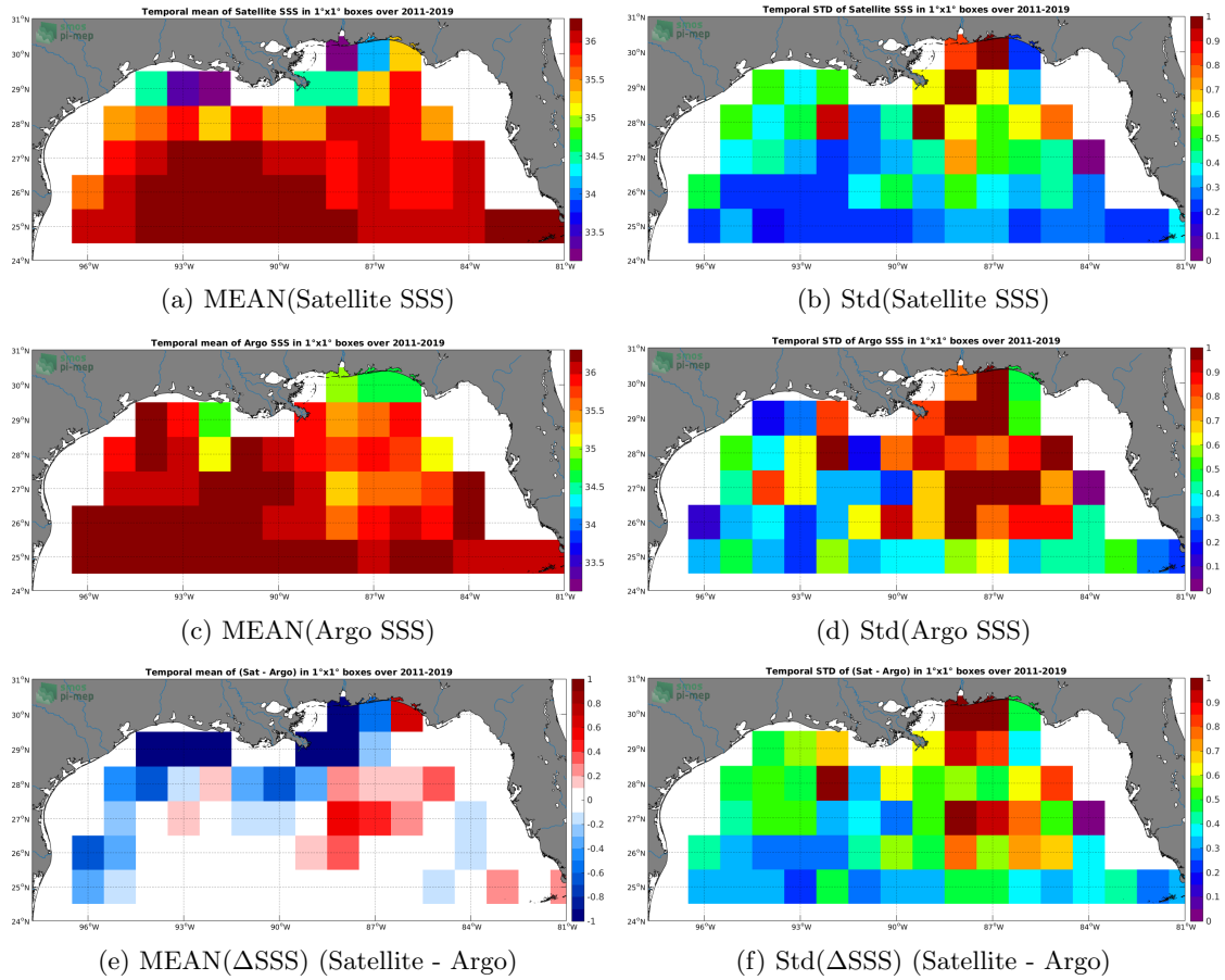
Figure 6: Temporal mean (left) and Std (right) of SSS from SMOS L3 v2 - 9-Days (BEC) (top), Argo (middle), and of \Delta SSS (Satellite - Argo). Only match-up pairs are used to generate these maps.
