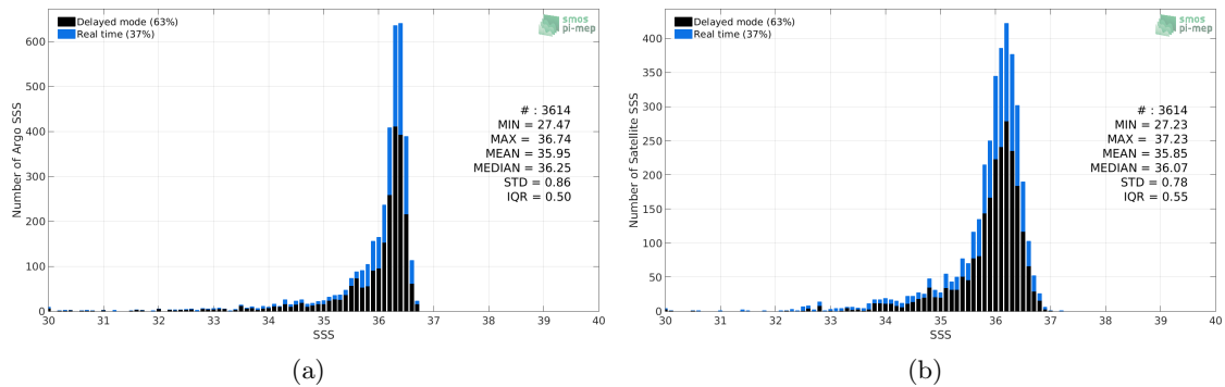
Figure 2: Histograms of SSS from Argo (a) and SMOS L3 v2 - 9-Days (BEC) (b) considering all match-up pairs per bins of 0.1 over the Mississippi river plume Pi-MEP region and for the full satellite product period.
