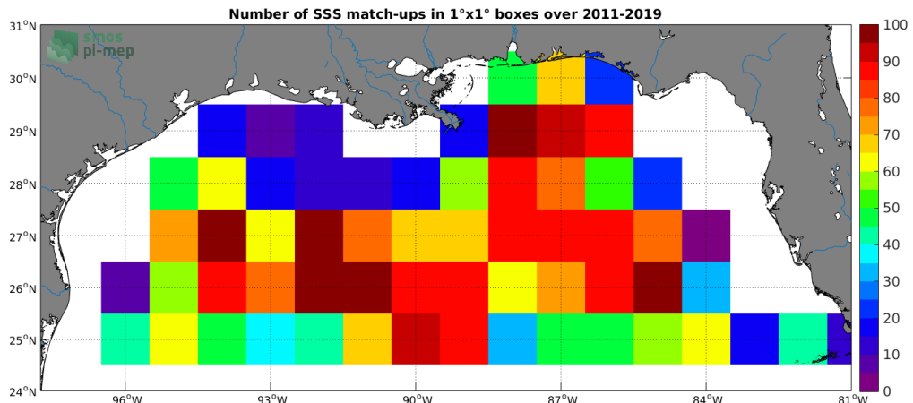
Figure 4: Number of SSS match-ups between Argo SSS and the SMOS L3 v2 - 9-Days (BEC) SSS product for the Mississippi river plume Pi-MEP region over 1^\circ \times 1^\circ boxes and for the full satellite product period.
